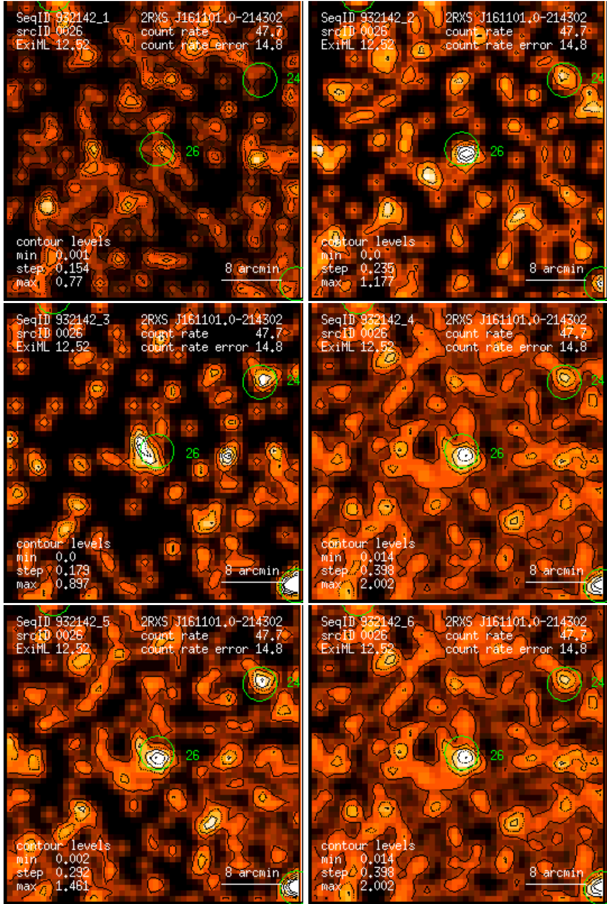
Figure 26: RASS 932142: detection 0026: band rate images, Gaussian filter: (1) PSPC channels 11 – 41, (2) 52 – 90, (3) 91 – 201, (4) 11 – 235, (5) 52 – 201, (6) 11 – 201. Broad band rates in counts/ks. Band rate contour levels in counts/ks/arcmin 2 .
