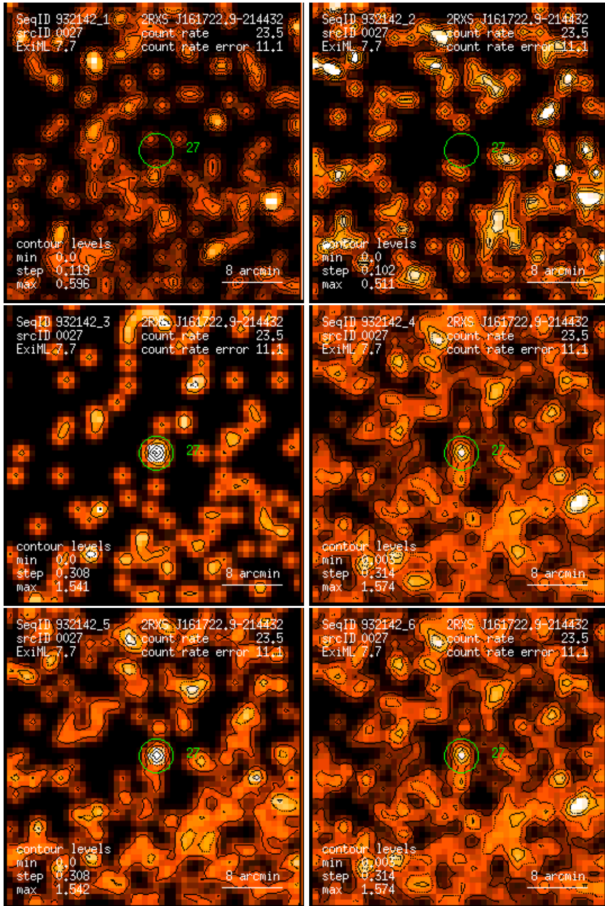
Figure 27: RASS 932142: detection 0027: band rate images, Gaussian filter: (1) PSPC channels 11 – 41, (2) 52 – 90, (3) 91 – 201, (4) 11 – 235, (5) 52 – 201, (6) 11 – 201. Broad band rates in counts/ks. Band rate contour levels in counts/ks/arcmin 2 .
