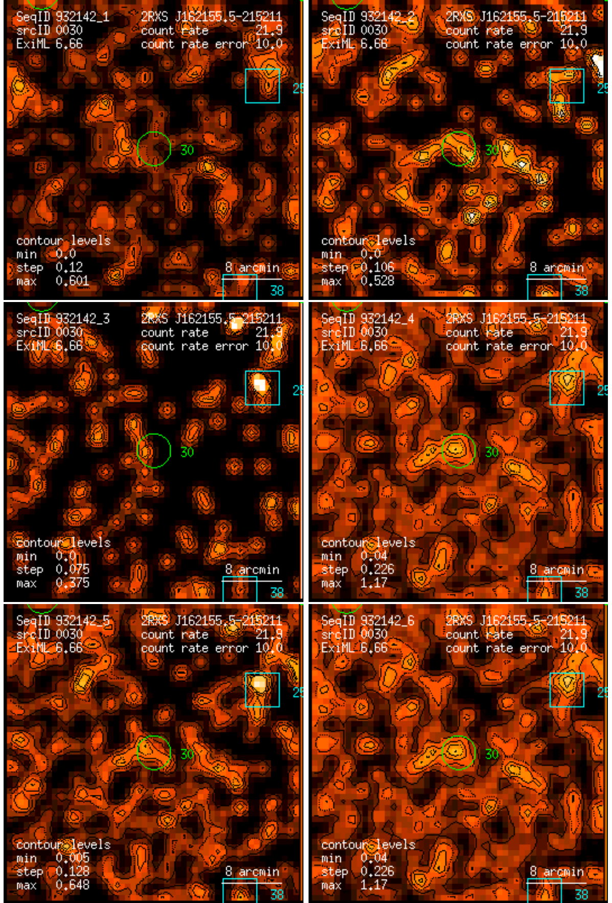
Figure 30: RASS 932142: detection 0030: band rate images, Gaussian filter: (1) PSPC channels 11 – 41, (2) 52 – 90, (3) 91 – 201, (4) 11 – 235, (5) 52 – 201, (6) 11 – 201. Broad band rates in counts/ks. Band rate contour levels in counts/ks/arcmin 2 .
