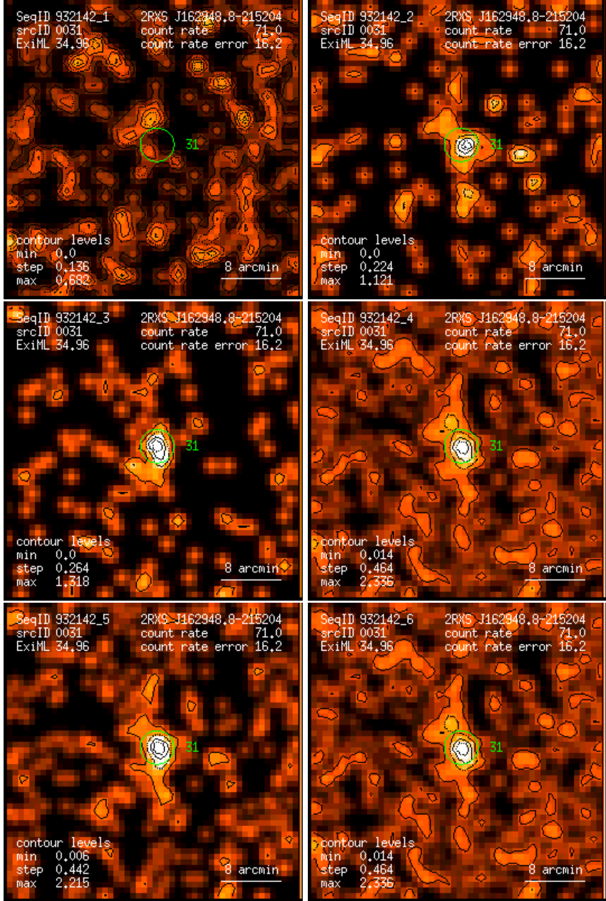
Figure 31: RASS 932142: detection 0031: band rate images, Gaussian filter: (1) PSPC channels 11 – 41, (2) 52 – 90, (3) 91 – 201, (4) 11 – 235, (5) 52 – 201, (6) 11 – 201. Broad band rates in counts/ks. Band rate contour levels in counts/ks/arcmin 2 .
