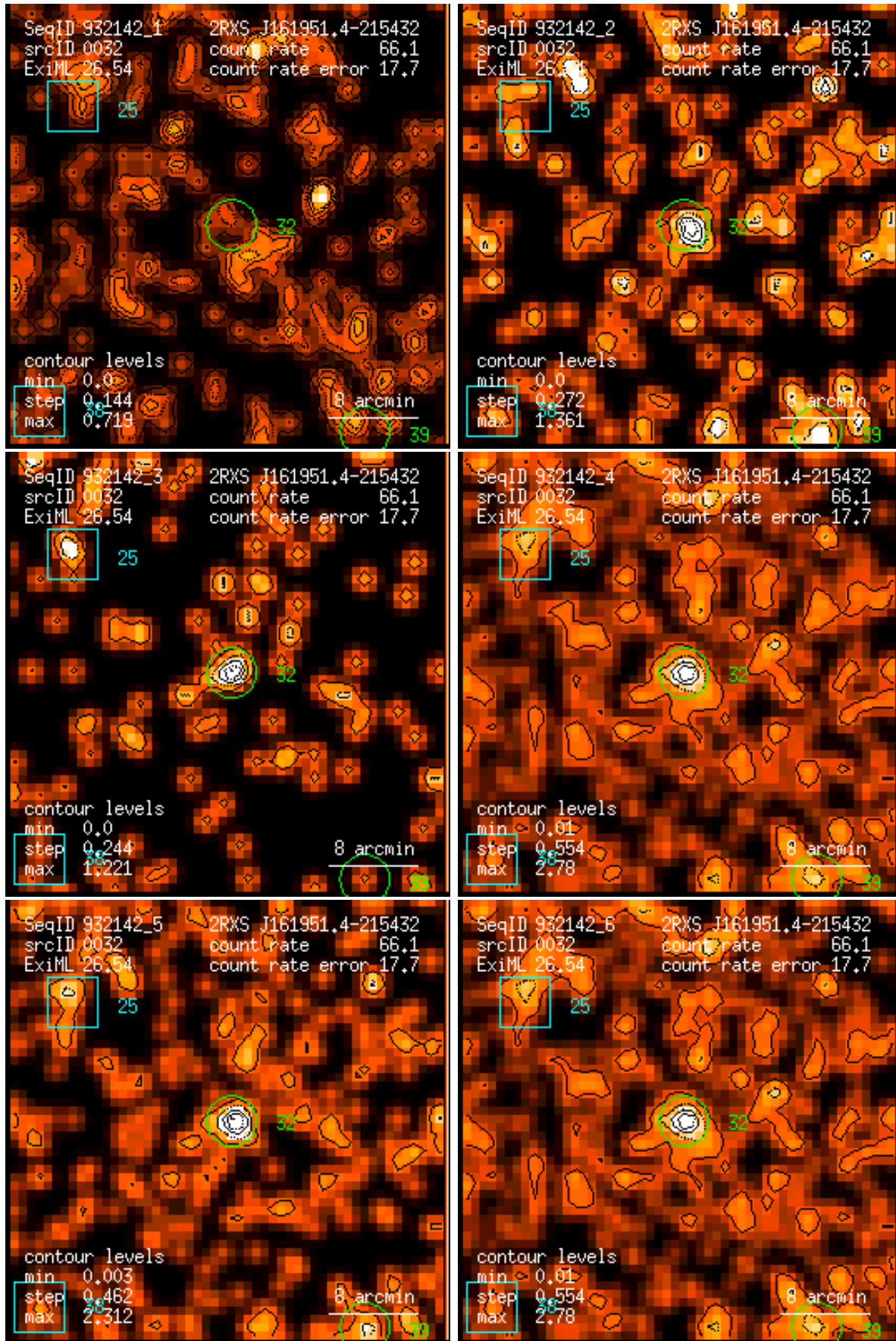
Figure 32: RASS 932142: detection 0032: band rate images, Gaussian filter: (1) PSPC channels 11 – 41, (2) 52 – 90, (3) 91 – 201, (4) 11 – 235, (5) 52 – 201, (6) 11 – 201. Broad band rates in counts/ks. Band rate contour levels in counts/ks/arcmin 2 .
