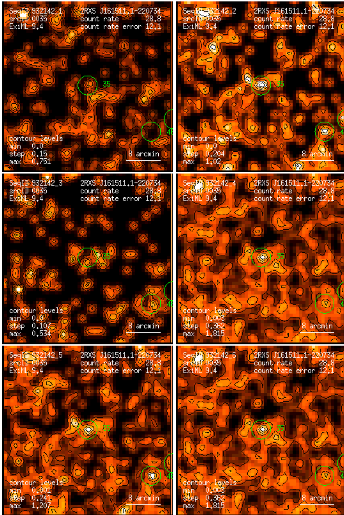
Figure 35: RASS 932142: detection 0035: band rate images, Gaussian filter: (1) PSPC channels 11 – 41, (2) 52 – 90, (3) 91 – 201, (4) 11 – 235, (5) 52 – 201, (6) 11 – 201. Broad band rates in counts/ks. Band rate contour levels in counts/ks/arcmin 2 .
