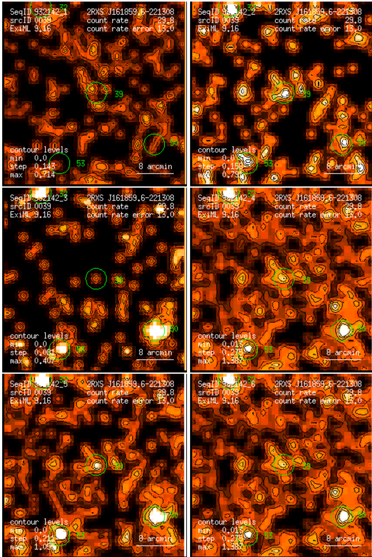
Figure 39: RASS 932142: detection 0039: band rate images, Gaussian filter: (1) PSPC channels 11 – 41, (2) 52 – 90, (3) 91 – 201, (4) 11 – 235, (5) 52 – 201, (6) 11 – 201. Broad band rates in counts/ks. Band rate contour levels in counts/ks/arcmin 2 .
