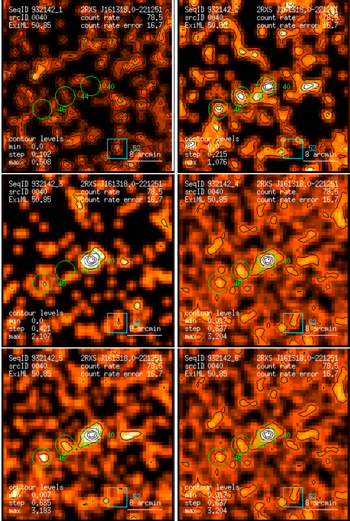
Figure 40: RASS 932142: detection 0040: band rate images, Gaussian filter: (1) PSPC channels 11 – 41, (2) 52 – 90, (3) 91 – 201, (4) 11 – 235, (5) 52 – 201, (6) 11 – 201. Broad band rates in counts/ks. Band rate contour levels in counts/ks/arcmin 2 .
