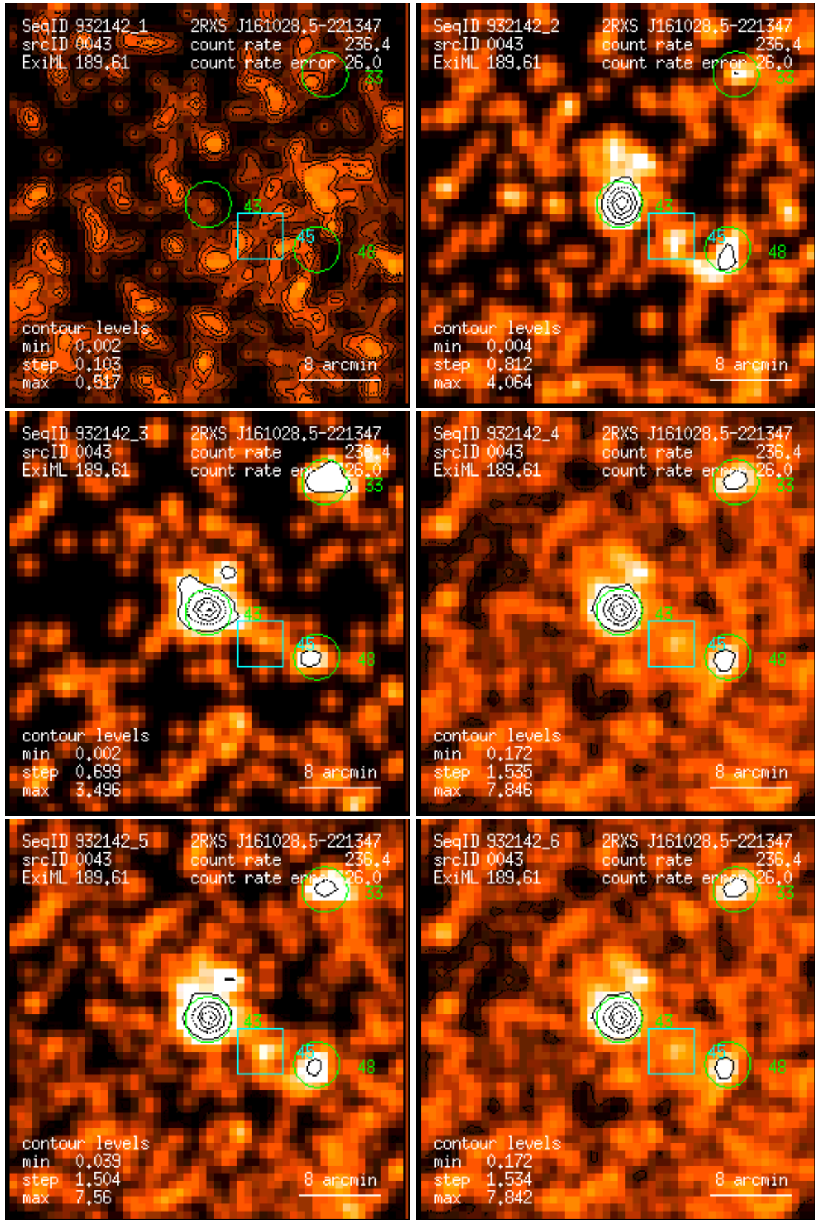
Figure 43: RASS 932142: detection 0043: band rate images, Gaussian filter: (1) PSPC channels 11 – 41, (2) 52 – 90, (3) 91 – 201, (4) 11 – 235, (5) 52 – 201, (6) 11 – 201. Broad band rates in counts/ks. Band rate contour levels in counts/ks/arcmin 2 .
