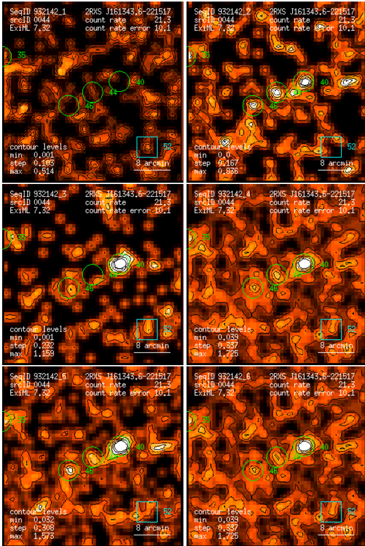
Figure 44: RASS 932142: detection 0044: band rate images, Gaussian filter: (1) PSPC channels 11 – 41, (2) 52 – 90, (3) 91 – 201, (4) 11 – 235, (5) 52 – 201, (6) 11 – 201. Broad band rates in counts/ks. Band rate contour levels in counts/ks/arcmin 2 .
