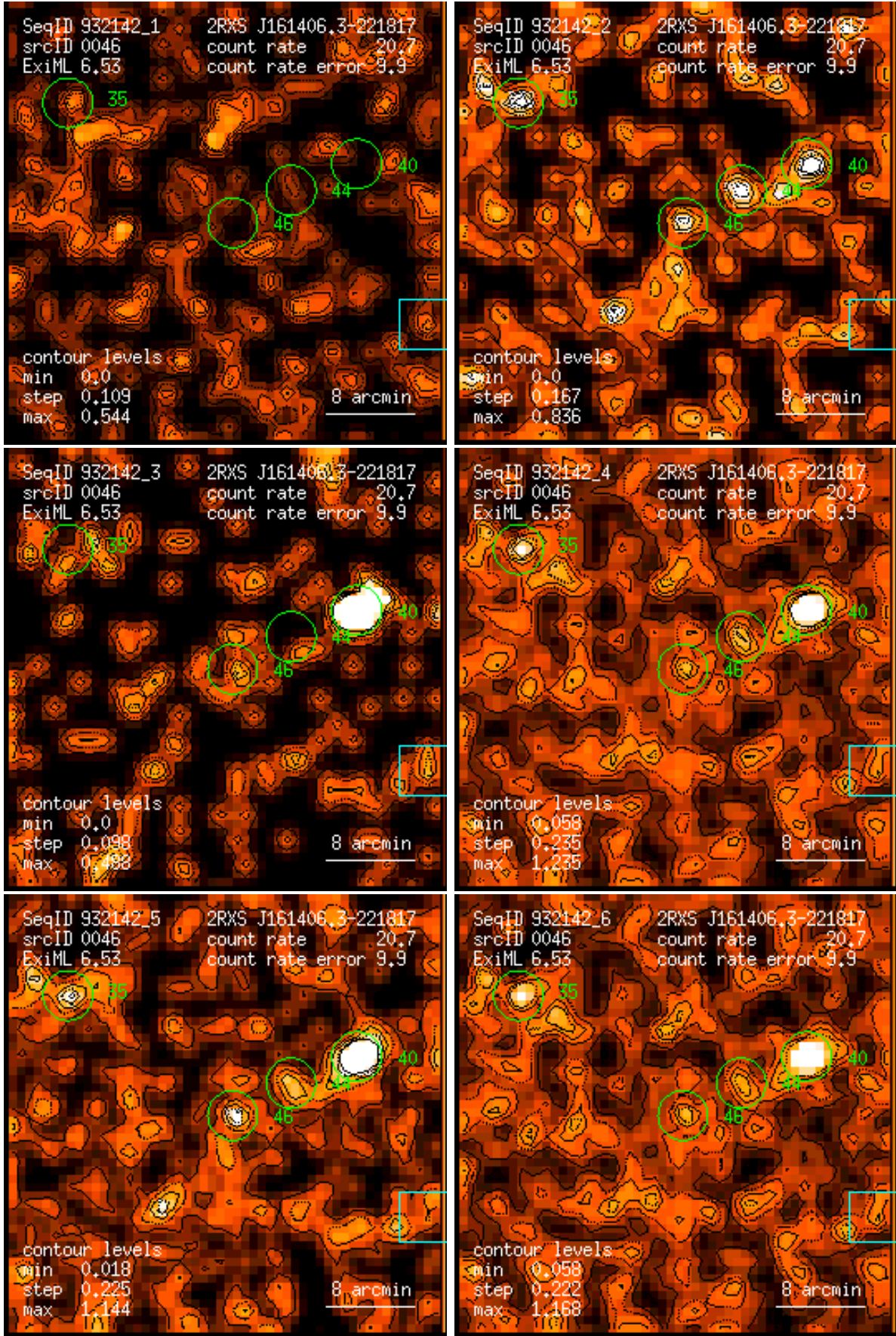
Figure 46: RASS 932142: detection 0046: band rate images, Gaussian filter: (1) PSPC channels 11 – 41, (2) 52 – 90, (3) 91 – 201, (4) 11 – 235, (5) 52 – 201, (6) 11 – 201. Broad band rates in counts/ks. Band rate contour levels in counts/ks/arcmin 2 .
