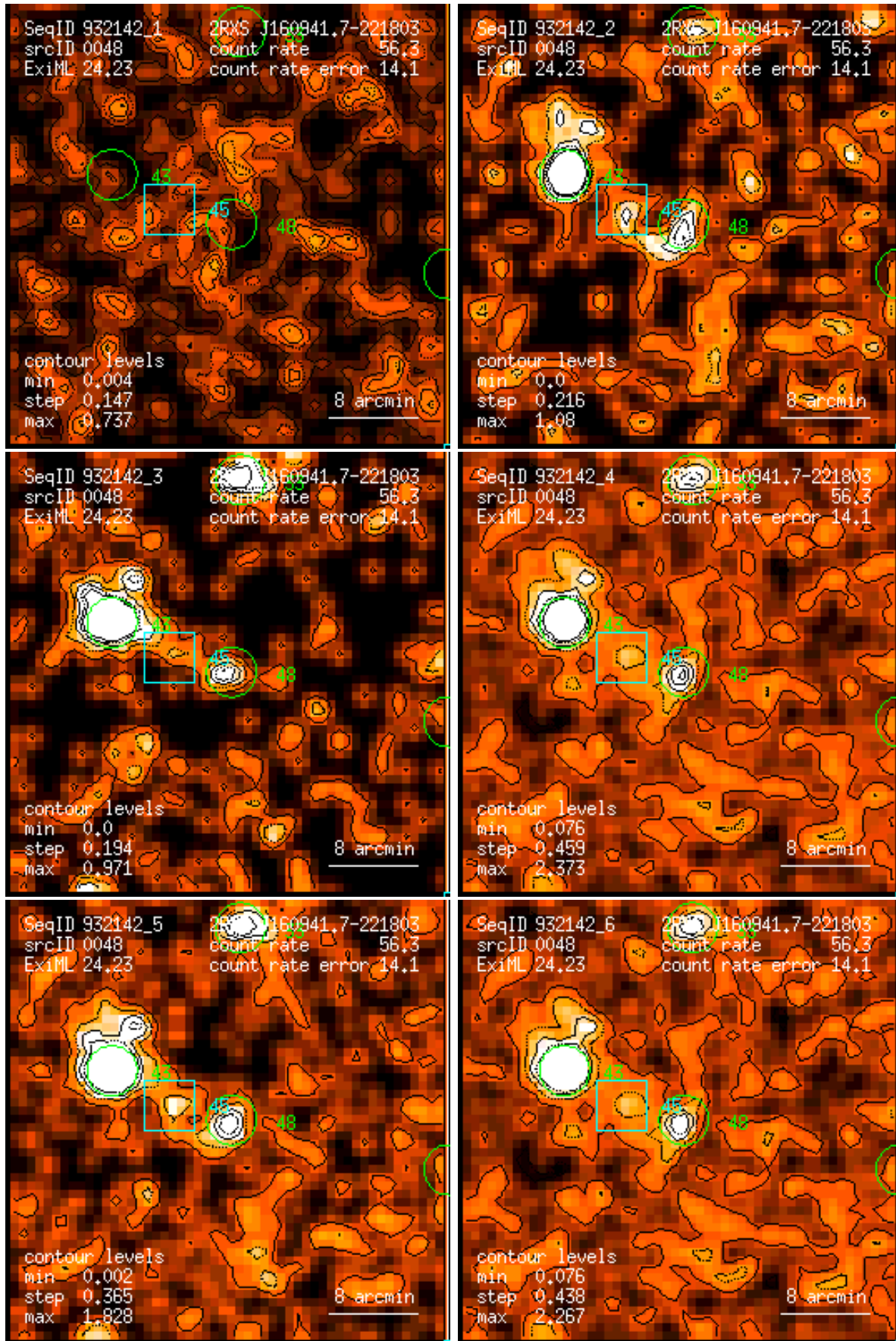
Figure 48: RASS 932142: detection 0048: band rate images, Gaussian filter: (1) PSPC channels 11 – 41, (2) 52 – 90, (3) 91 – 201, (4) 11 – 235, (5) 52 – 201, (6) 11 – 201. Broad band rates in counts/ks. Band rate contour levels in counts/ks/arcmin 2 .
