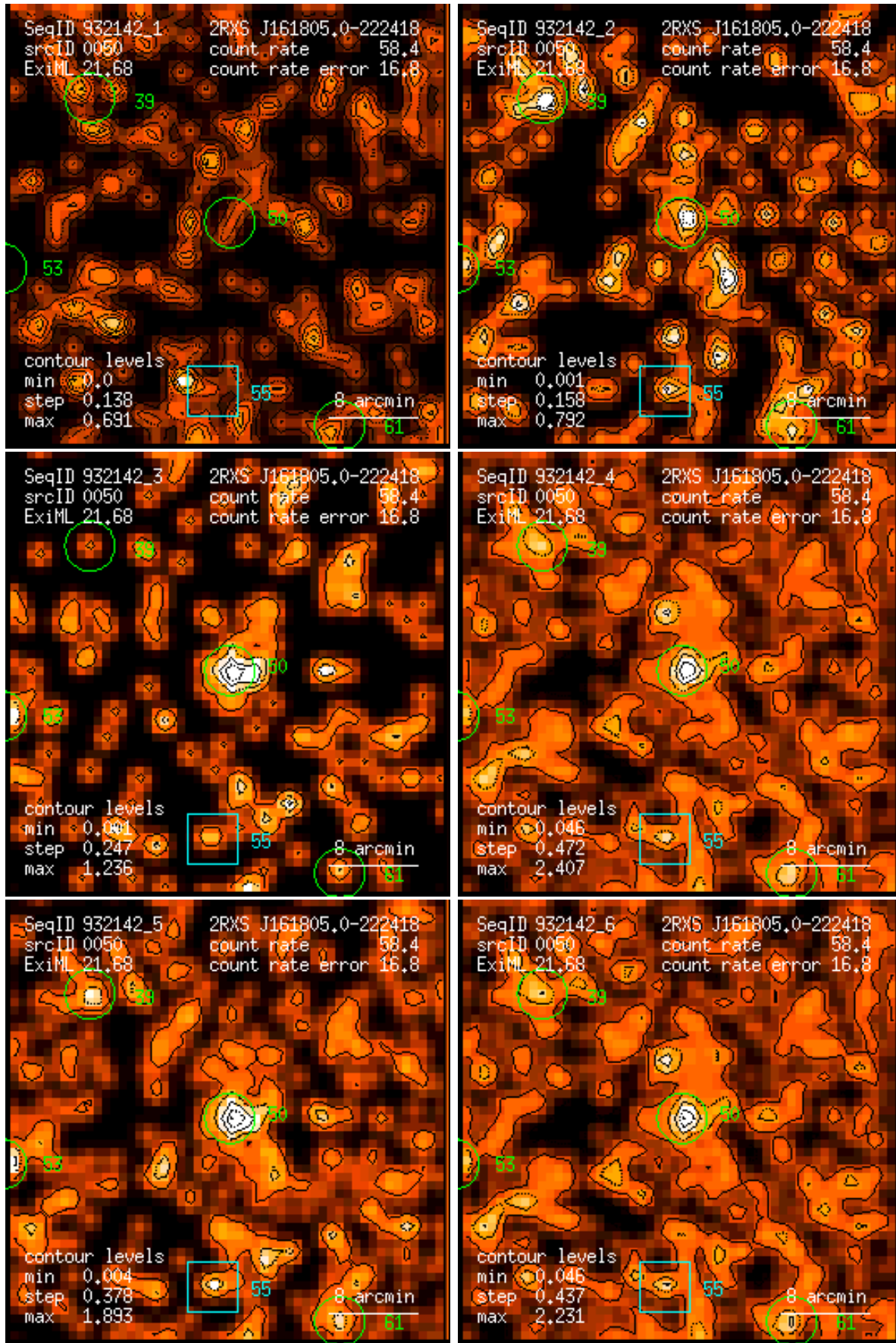
Figure 50: RASS 932142: detection 0050: band rate images, Gaussian filter: (1) PSPC channels 11 – 41, (2) 52 – 90, (3) 91 – 201, (4) 11 – 235, (5) 52 – 201, (6) 11 – 201. Broad band rates in counts/ks. Band rate contour levels in counts/ks/arcmin 2 .
