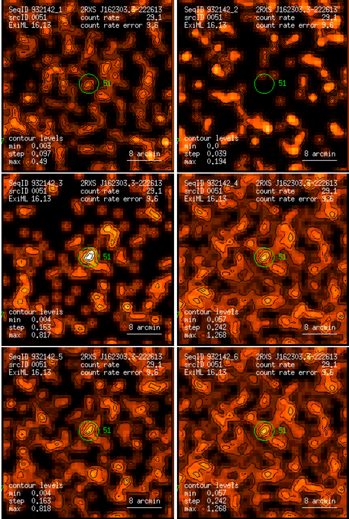
Figure 51: RASS 932142: detection 0051: band rate images, Gaussian filter: (1) PSPC channels 11 – 41, (2) 52 – 90, (3) 91 – 201, (4) 11 – 235, (5) 52 – 201, (6) 11 – 201. Broad band rates in counts/ks. Band rate contour levels in counts/ks/arcmin 2 .
