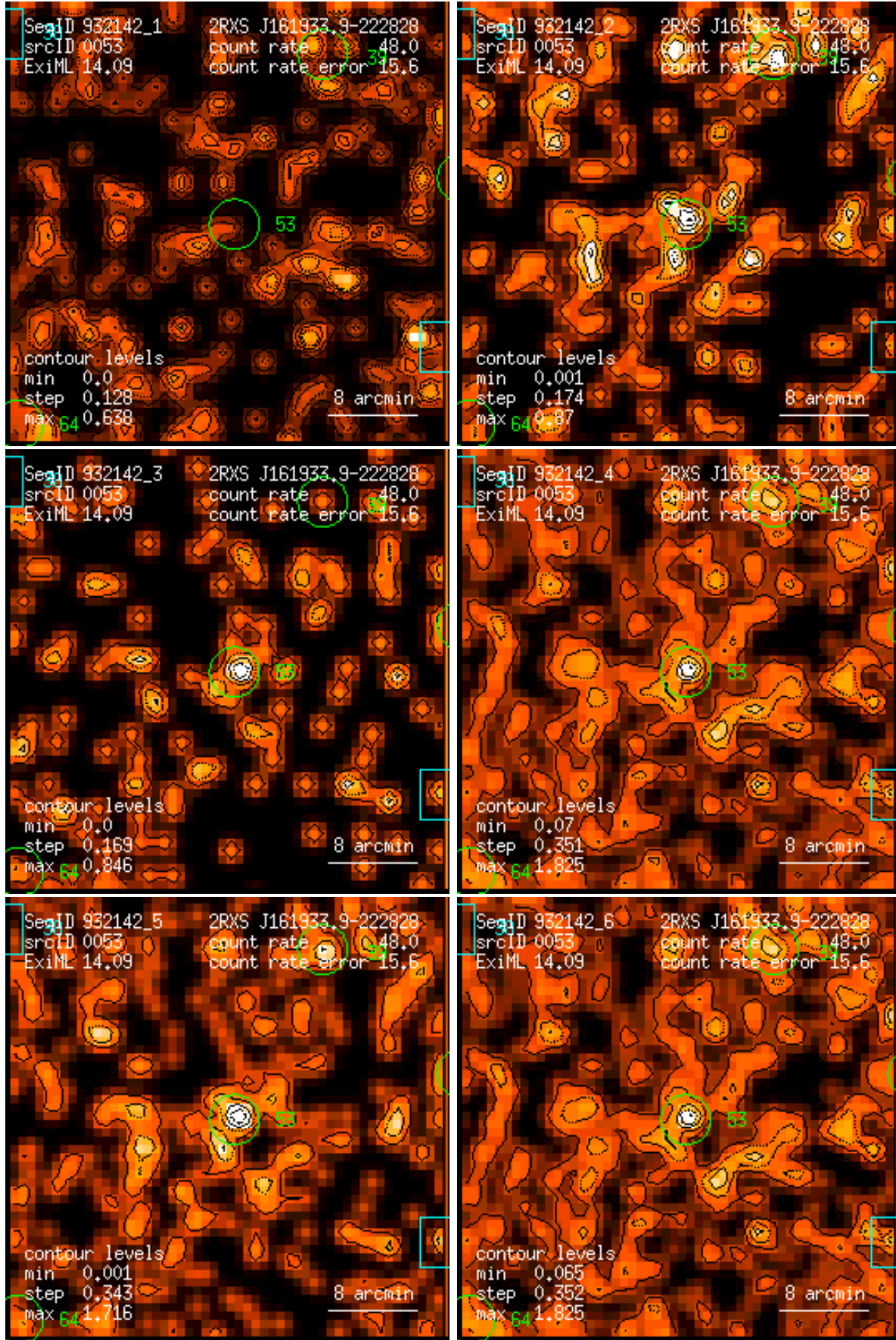
Figure 53: RASS 932142: detection 0053: band rate images, Gaussian filter: (1) PSPC channels 11 – 41, (2) 52 – 90, (3) 91 – 201, (4) 11 – 235, (5) 52 – 201, (6) 11 – 201. Broad band rates in counts/ks. Band rate contour levels in counts/ks/arcmin 2 .
