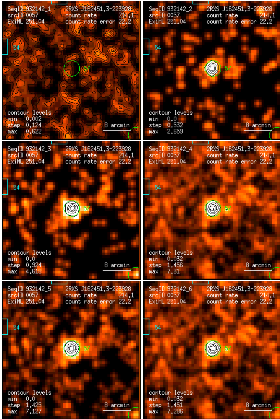
Figure 57: RASS 932142: detection 0057: band rate images, Gaussian filter: (1) PSPC channels 11 – 41, (2) 52 – 90, (3) 91 – 201, (4) 11 – 235, (5) 52 – 201, (6) 11 – 201. Broad band rates in counts/ks. Band rate contour levels in counts/ks/arcmin 2 .
