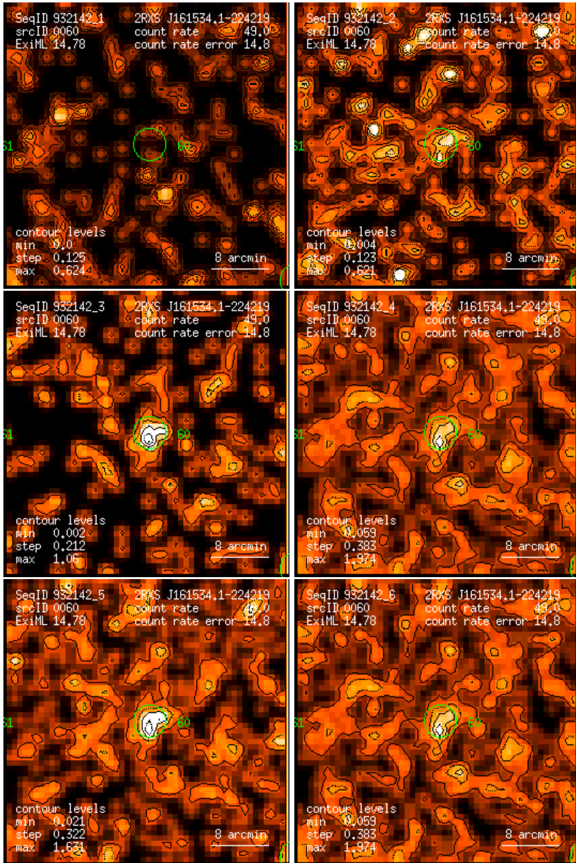
Figure 60: RASS 932142: detection 0060: band rate images, Gaussian filter: (1) PSPC channels 11 – 41, (2) 52 – 90, (3) 91 – 201, (4) 11 – 235, (5) 52 – 201, (6) 11 – 201. Broad band rates in counts/ks. Band rate contour levels in counts/ks/arcmin 2 .
