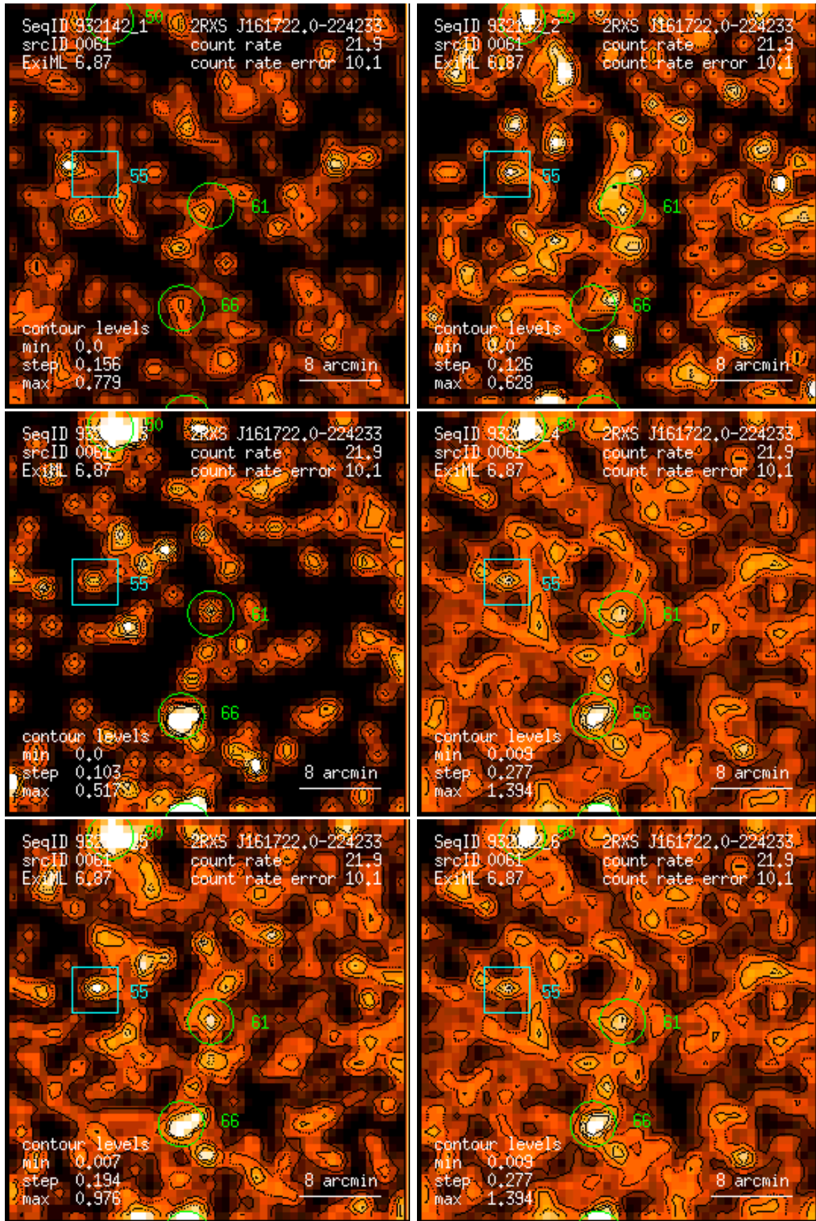
Figure 61: RASS 932142: detection 0061: band rate images, Gaussian filter: (1) PSPC channels 11 – 41, (2) 52 – 90, (3) 91 – 201, (4) 11 – 235, (5) 52 – 201, (6) 11 – 201. Broad band rates in counts/ks. Band rate contour levels in counts/ks/arcmin 2 .
