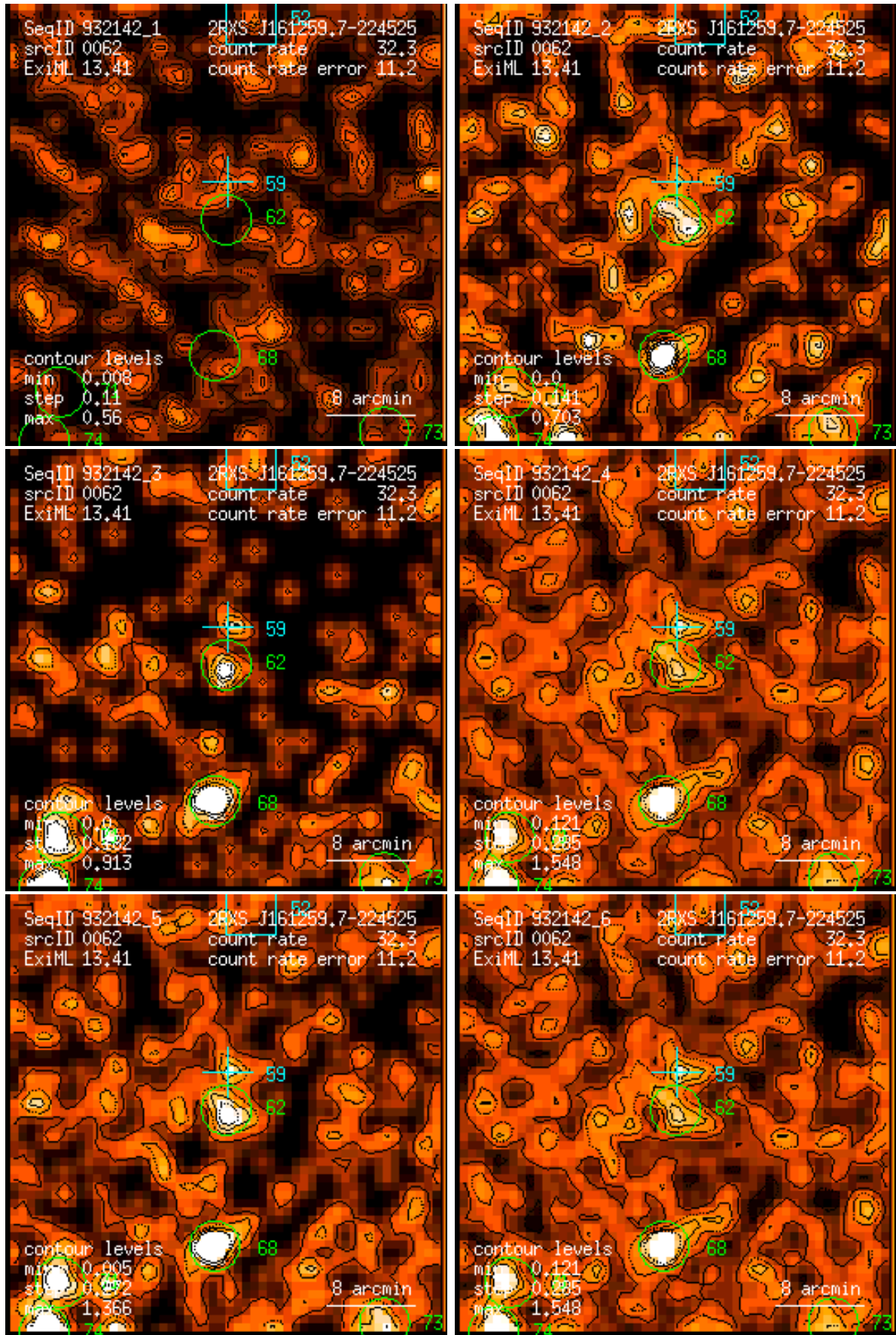
Figure 62: RASS 932142: detection 0062: band rate images, Gaussian filter: (1) PSPC channels 11 – 41, (2) 52 – 90, (3) 91 – 201, (4) 11 – 235, (5) 52 – 201, (6) 11 – 201. Broad band rates in counts/ks. Band rate contour levels in counts/ks/arcmin 2 .
