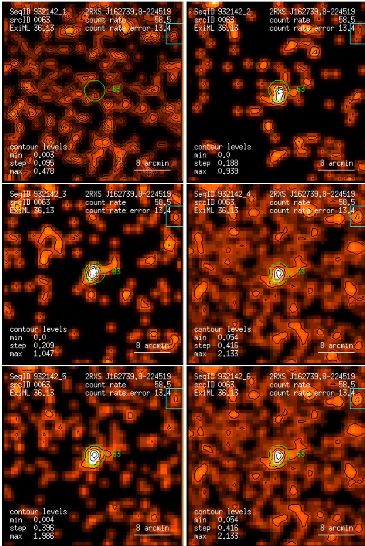
Figure 63: RASS 932142: detection 0063: band rate images, Gaussian filter: (1) PSPC channels 11 – 41, (2) 52 – 90, (3) 91 – 201, (4) 11 – 235, (5) 52 – 201, (6) 11 – 201. Broad band rates in counts/ks. Band rate contour levels in counts/ks/arcmin 2 .
