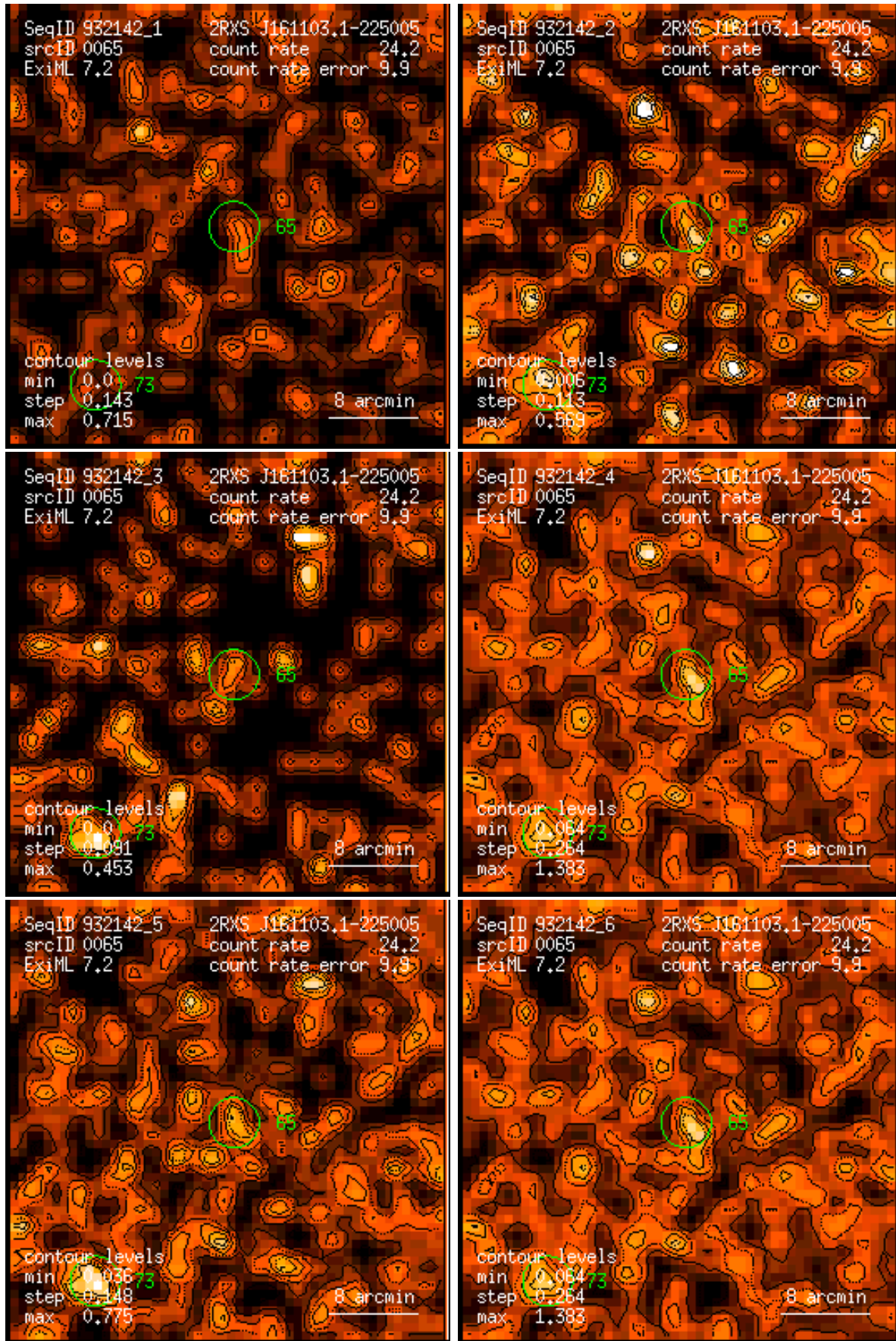
Figure 65: RASS 932142: detection 0065: band rate images, Gaussian filter: (1) PSPC channels 11 – 41, (2) 52 – 90, (3) 91 – 201, (4) 11 – 235, (5) 52 – 201, (6) 11 – 201. Broad band rates in counts/ks. Band rate contour levels in counts/ks/arcmin 2 .
