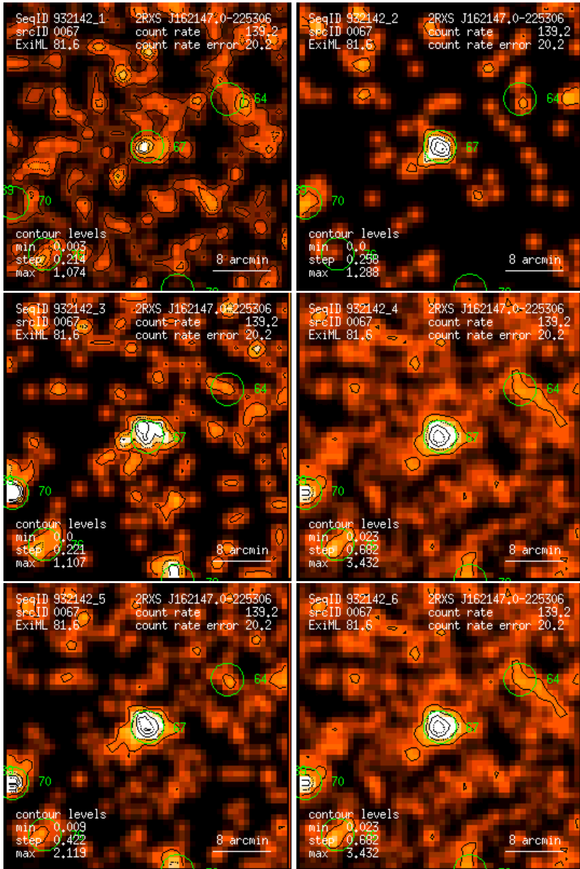
Figure 67: RASS 932142: detection 0067: band rate images, Gaussian filter: (1) PSPC channels 11 – 41, (2) 52 – 90, (3) 91 – 201, (4) 11 – 235, (5) 52 – 201, (6) 11 – 201. Broad band rates in counts/ks. Band rate contour levels in counts/ks/arcmin 2 .
