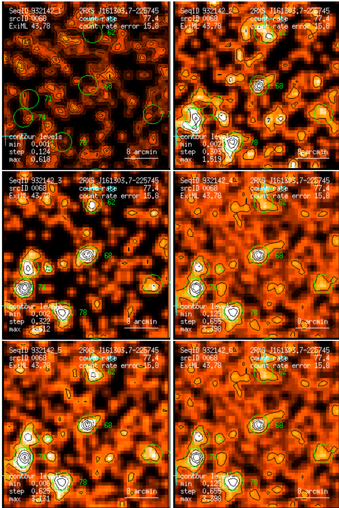
Figure 68: RASS 932142: detection 0068: band rate images, Gaussian filter: (1) PSPC channels 11 – 41, (2) 52 – 90, (3) 91 – 201, (4) 11 – 235, (5) 52 – 201, (6) 11 – 201. Broad band rates in counts/ks. Band rate contour levels in counts/ks/arcmin 2 .
