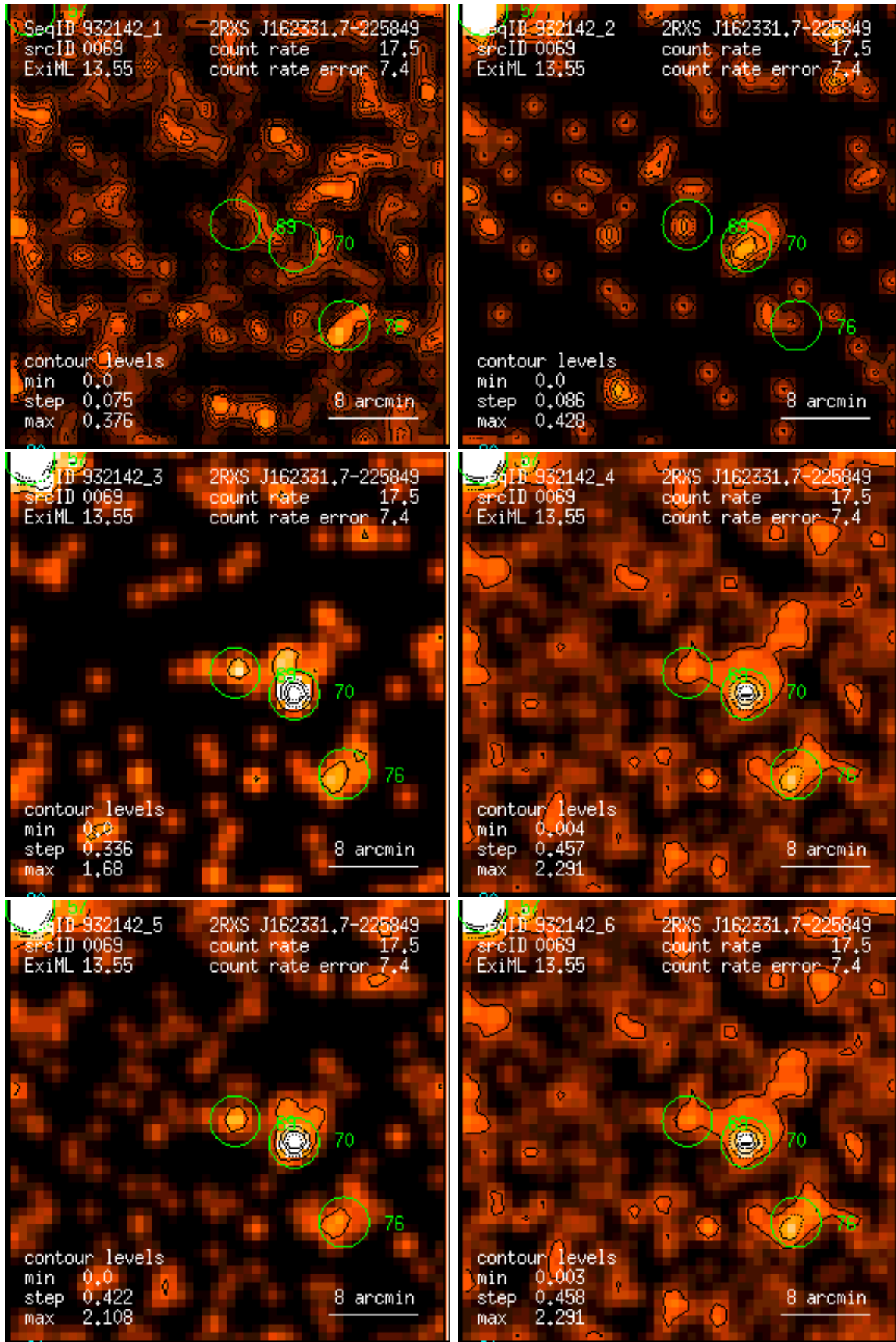
Figure 69: RASS 932142: detection 0069: band rate images, Gaussian filter: (1) PSPC channels 11 – 41, (2) 52 – 90, (3) 91 – 201, (4) 11 – 235, (5) 52 – 201, (6) 11 – 201. Broad band rates in counts/ks. Band rate contour levels in counts/ks/arcmin 2 .
