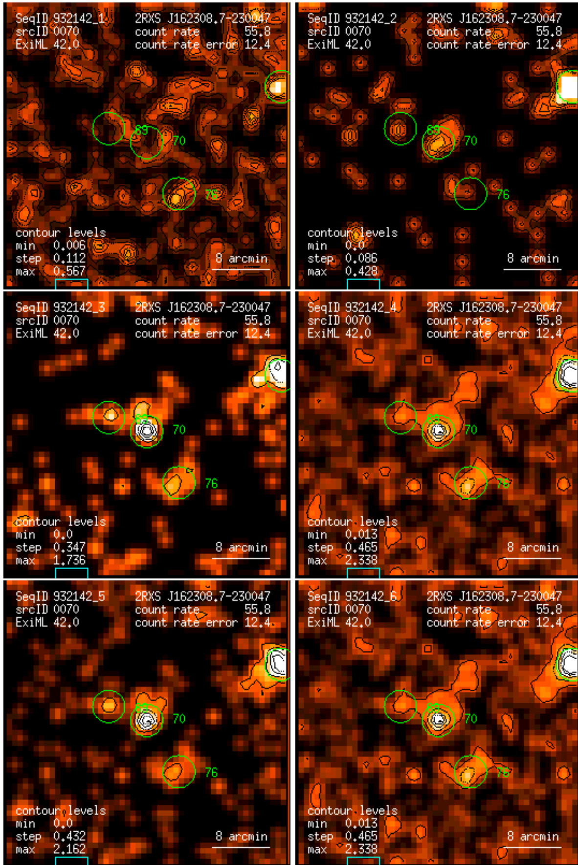
Figure 70: RASS 932142: detection 0070: band rate images, Gaussian filter: (1) PSPC channels 11 – 41, (2) 52 – 90, (3) 91 – 201, (4) 11 – 235, (5) 52 – 201, (6) 11 – 201. Broad band rates in counts/ks. Band rate contour levels in counts/ks/arcmin 2 .
