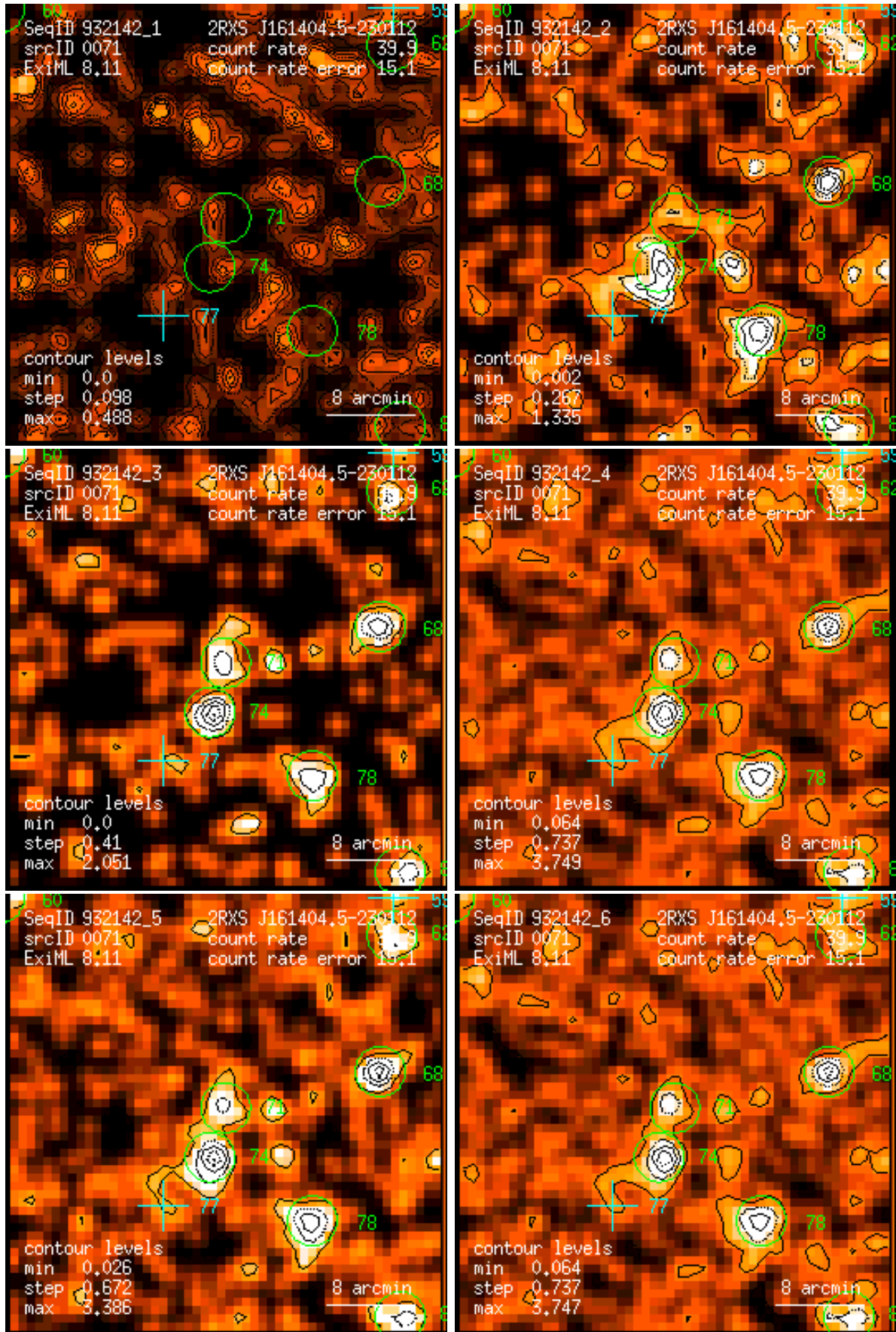
Figure 71: RASS 932142: detection 0071: band rate images, Gaussian filter: (1) PSPC channels 11 – 41, (2) 52 – 90, (3) 91 – 201, (4) 11 – 235, (5) 52 – 201, (6) 11 – 201. Broad band rates in counts/ks. Band rate contour levels in counts/ks/arcmin 2 .
