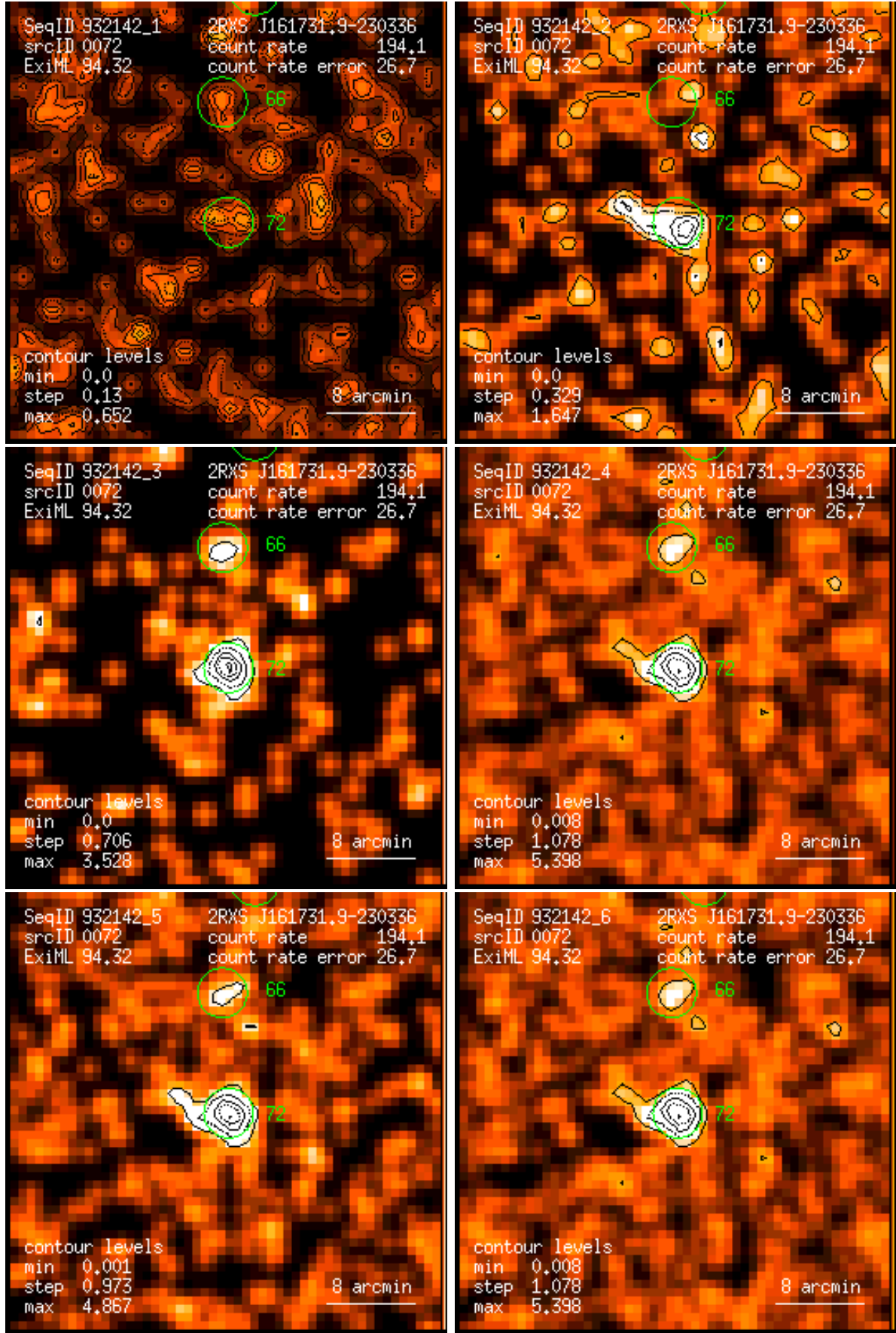
Figure 72: RASS 932142: detection 0072: band rate images, Gaussian filter: (1) PSPC channels 11 – 41, (2) 52 – 90, (3) 91 – 201, (4) 11 – 235, (5) 52 – 201, (6) 11 – 201. Broad band rates in counts/ks. Band rate contour levels in counts/ks/arcmin 2 .
