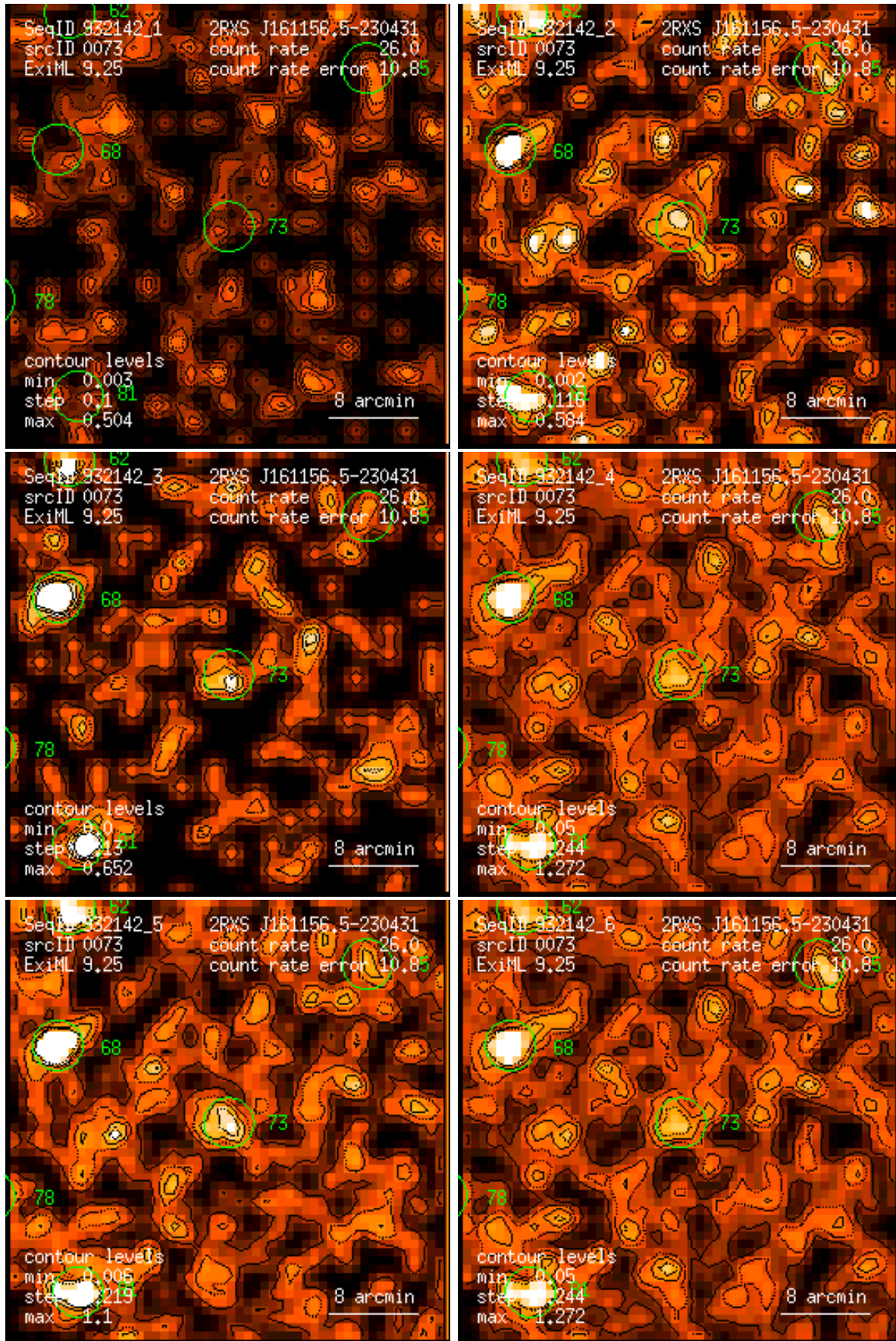
Figure 73: RASS 932142: detection 0073: band rate images, Gaussian filter: (1) PSPC channels 11 – 41, (2) 52 – 90, (3) 91 – 201, (4) 11 – 235, (5) 52 – 201, (6) 11 – 201. Broad band rates in counts/ks. Band rate contour levels in counts/ks/arcmin 2 .
