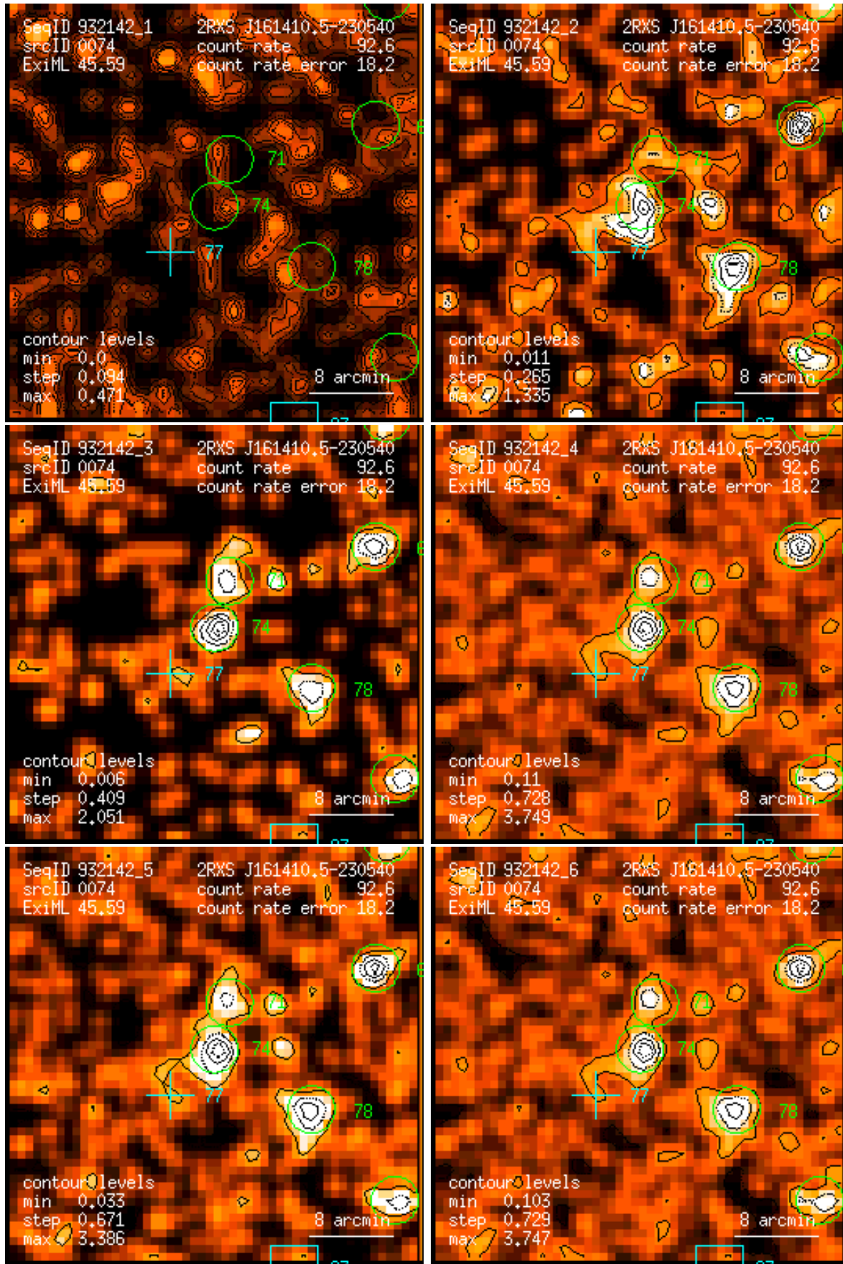
Figure 74: RASS 932142: detection 0074: band rate images, Gaussian filter: (1) PSPC channels 11 – 41, (2) 52 – 90, (3) 91 – 201, (4) 11 – 235, (5) 52 – 201, (6) 11 – 201. Broad band rates in counts/ks. Band rate contour levels in counts/ks/arcmin 2 .
