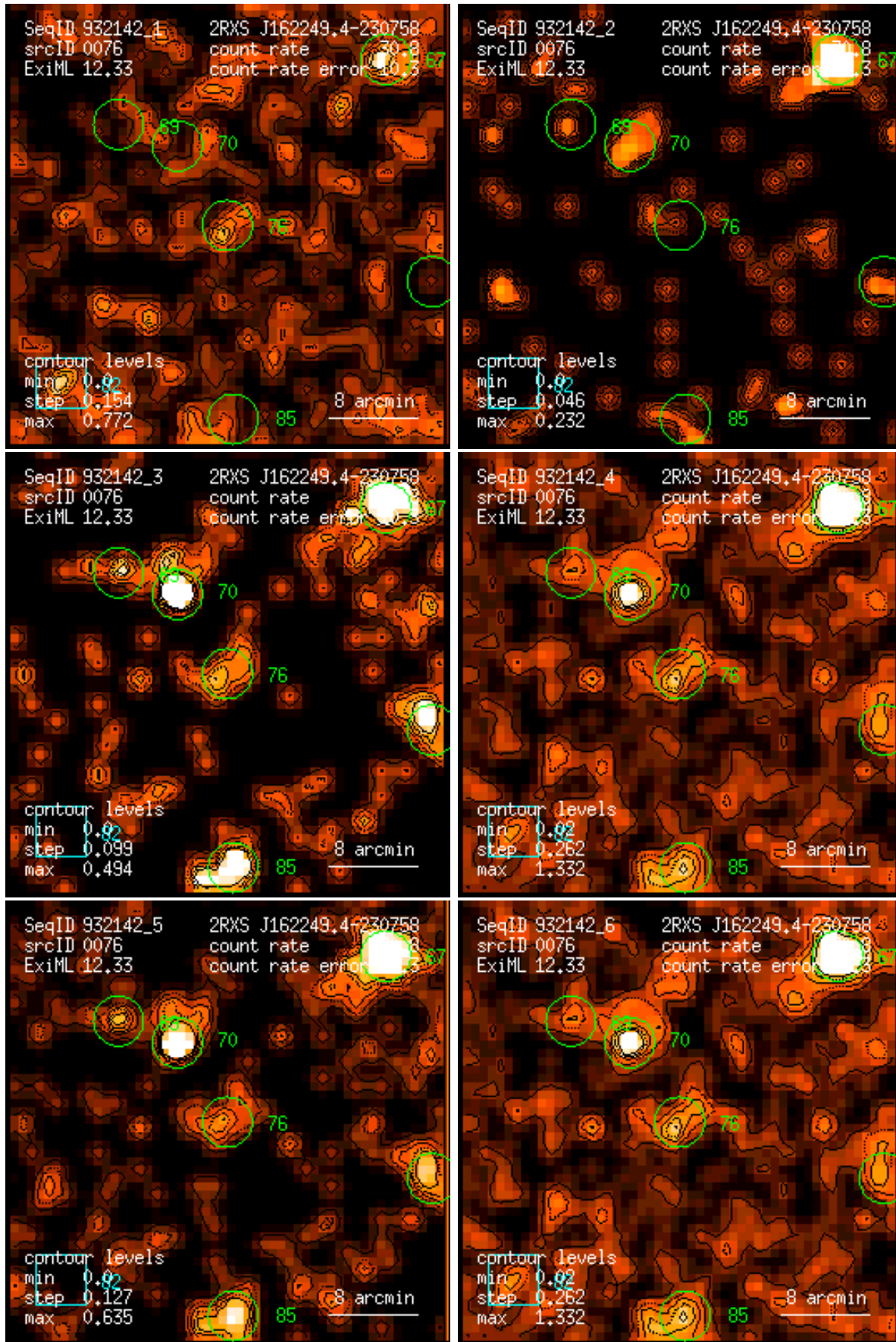
Figure 76: RASS 932142: detection 0076: band rate images, Gaussian filter: (1) PSPC channels 11 – 41, (2) 52 – 90, (3) 91 – 201, (4) 11 – 235, (5) 52 – 201, (6) 11 – 201. Broad band rates in counts/ks. Band rate contour levels in counts/ks/arcmin 2 .
