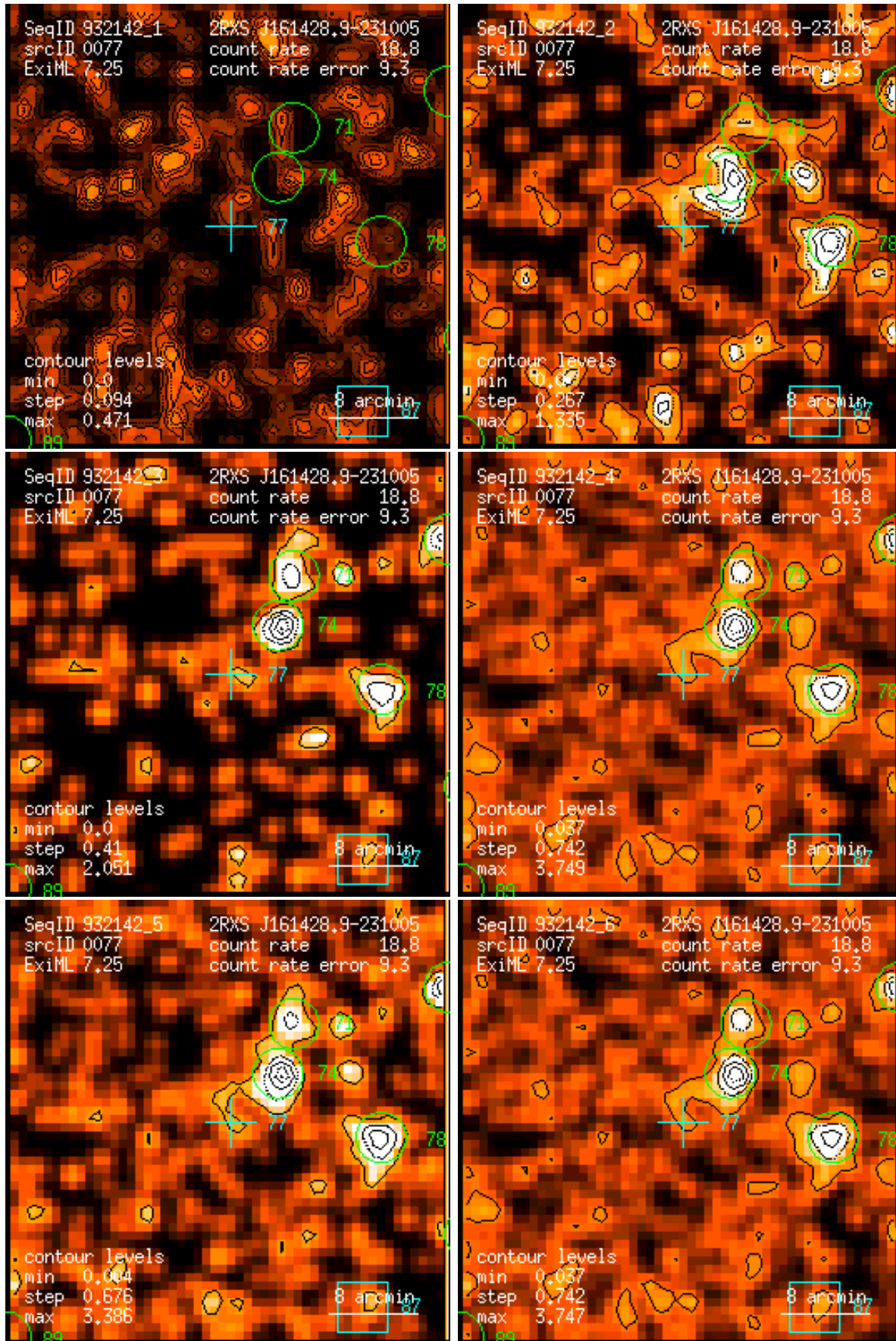
Figure 77: RASS 932142: detection 0077: band rate images, Gaussian filter: (1) PSPC channels 11 – 41, (2) 52 – 90, (3) 91 – 201, (4) 11 – 235, (5) 52 – 201, (6) 11 – 201. Broad band rates in counts/ks. Band rate contour levels in counts/ks/arcmin 2 .
