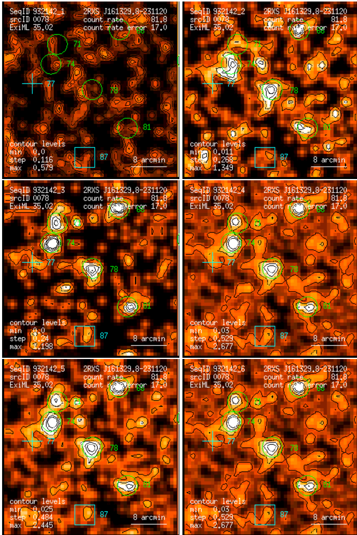
Figure 78: RASS 932142: detection 0078: band rate images, Gaussian filter: (1) PSPC channels 11 – 41, (2) 52 – 90, (3) 91 – 201, (4) 11 – 235, (5) 52 – 201, (6) 11 – 201. Broad band rates in counts/ks. Band rate contour levels in counts/ks/arcmin 2 .
