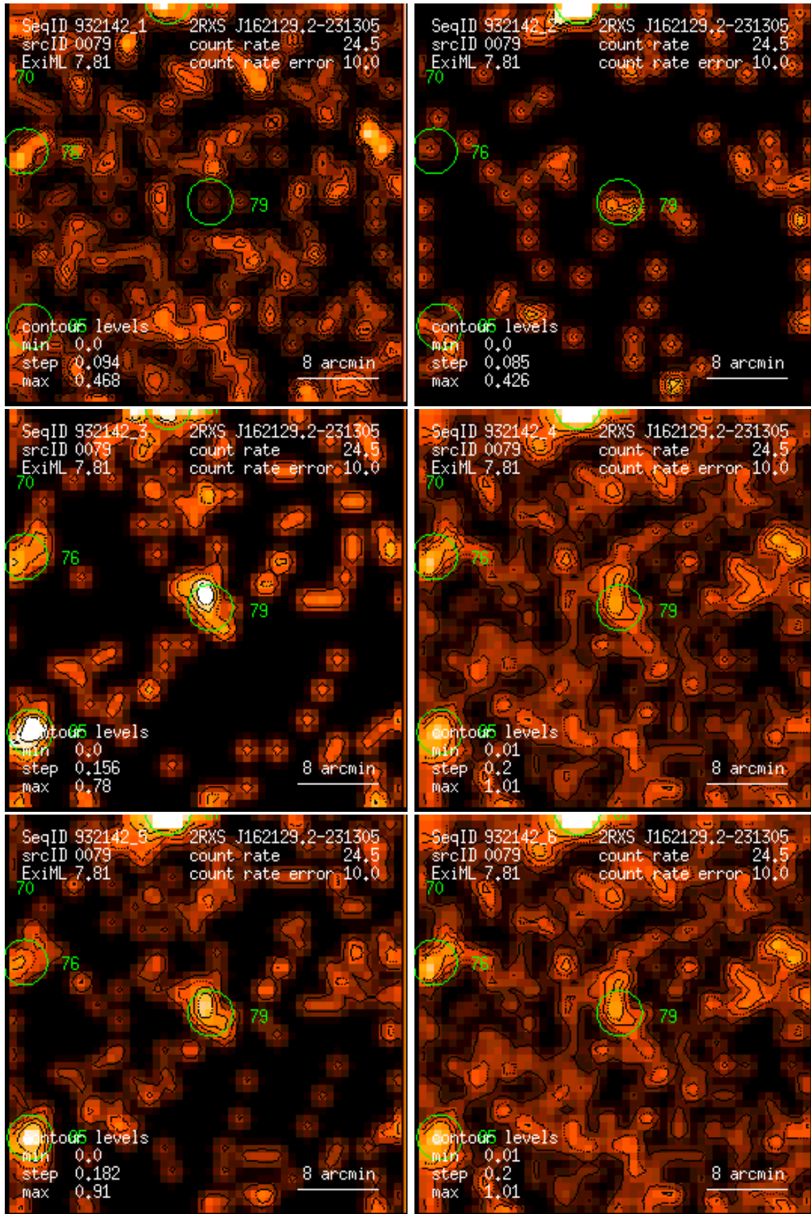
Figure 79: RASS 932142: detection 0079: band rate images, Gaussian filter: (1) PSPC channels 11 – 41, (2) 52 – 90, (3) 91 – 201, (4) 11 – 235, (5) 52 – 201, (6) 11 – 201. Broad band rates in counts/ks. Band rate contour levels in counts/ks/arcmin 2 .
