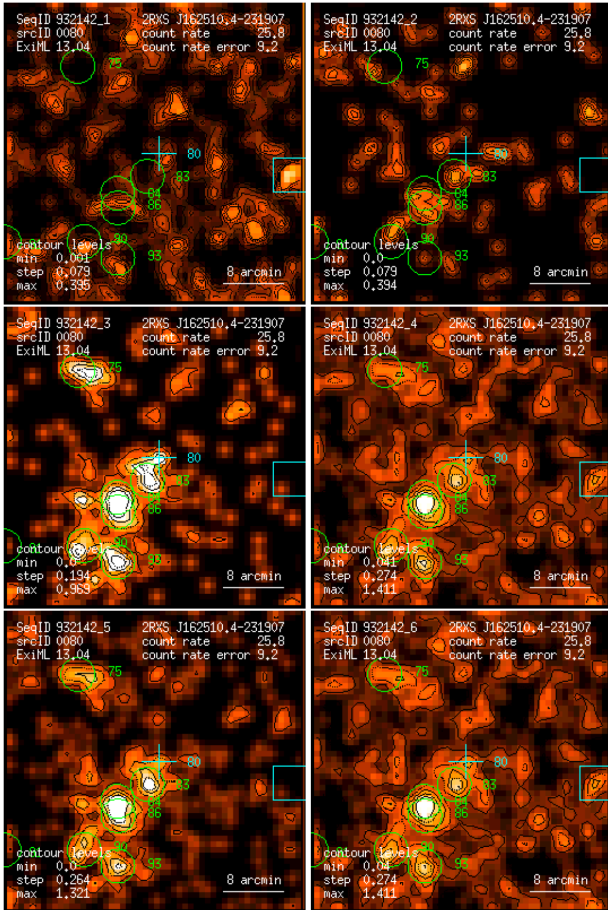
Figure 80: RASS 932142: detection 0080: band rate images, Gaussian filter: (1) PSPC channels 11 – 41, (2) 52 – 90, (3) 91 – 201, (4) 11 – 235, (5) 52 – 201, (6) 11 – 201. Broad band rates in counts/ks. Band rate contour levels in counts/ks/arcmin 2 .
