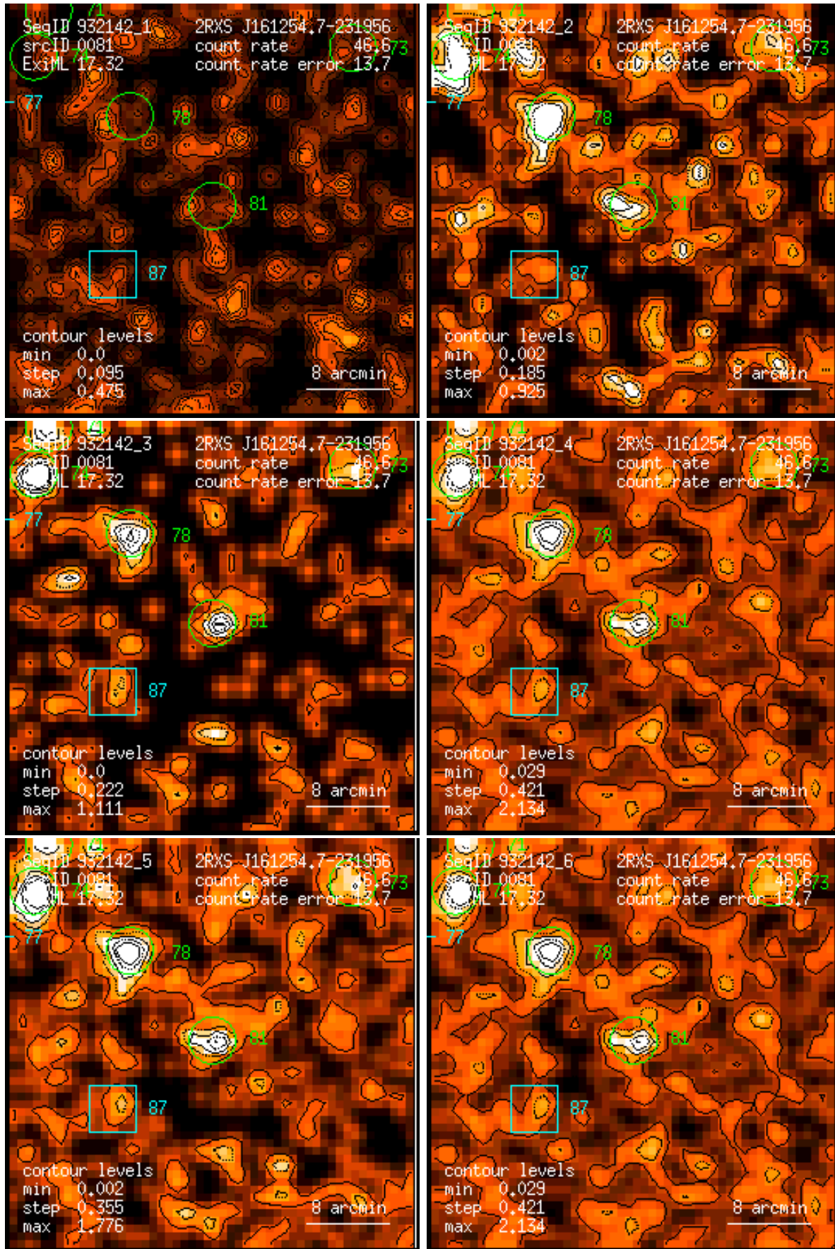
Figure 81: RASS 932142: detection 0081: band rate images, Gaussian filter: (1) PSPC channels 11 – 41, (2) 52 – 90, (3) 91 – 201, (4) 11 – 235, (5) 52 – 201, (6) 11 – 201. Broad band rates in counts/ks. Band rate contour levels in counts/ks/arcmin 2 .
