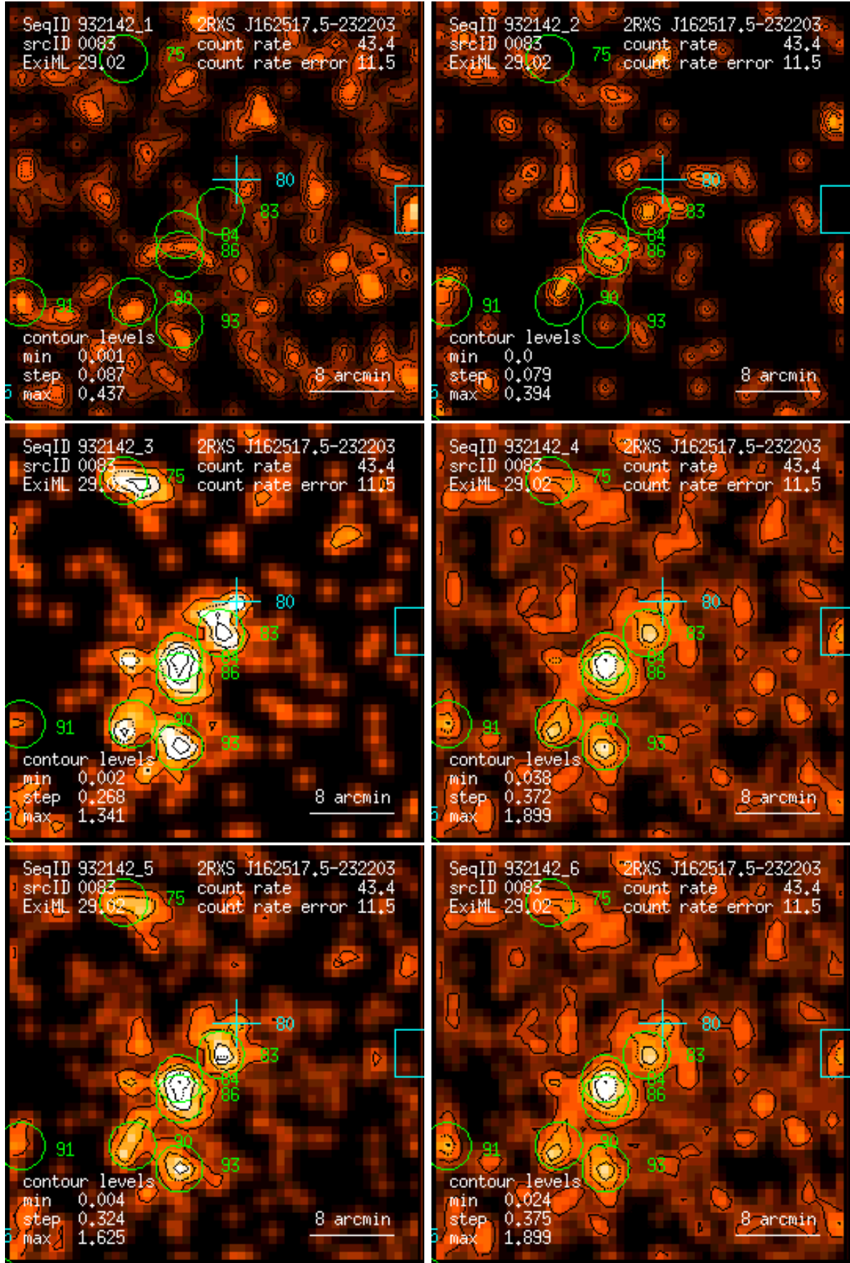
Figure 83: RASS 932142: detection 0083: band rate images, Gaussian filter: (1) PSPC channels 11 – 41, (2) 52 – 90, (3) 91 – 201, (4) 11 – 235, (5) 52 – 201, (6) 11 – 201. Broad band rates in counts/ks. Band rate contour levels in counts/ks/arcmin 2 .
