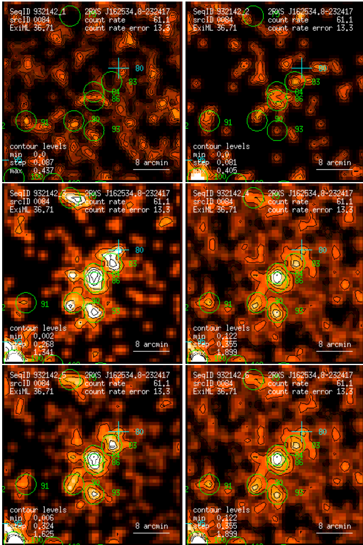
Figure 84: RASS 932142: detection 0084: band rate images, Gaussian filter: (1) PSPC channels 11 – 41, (2) 52 – 90, (3) 91 – 201, (4) 11 – 235, (5) 52 – 201, (6) 11 – 201. Broad band rates in counts/ks. Band rate contour levels in counts/ks/arcmin 2 .
