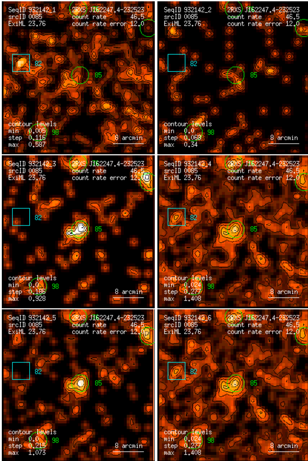
Figure 85: RASS 932142: detection 0085: band rate images, Gaussian filter: (1) PSPC channels 11 – 41, (2) 52 – 90, (3) 91 – 201, (4) 11 – 235, (5) 52 – 201, (6) 11 – 201. Broad band rates in counts/ks. Band rate contour levels in counts/ks/arcmin 2 .
