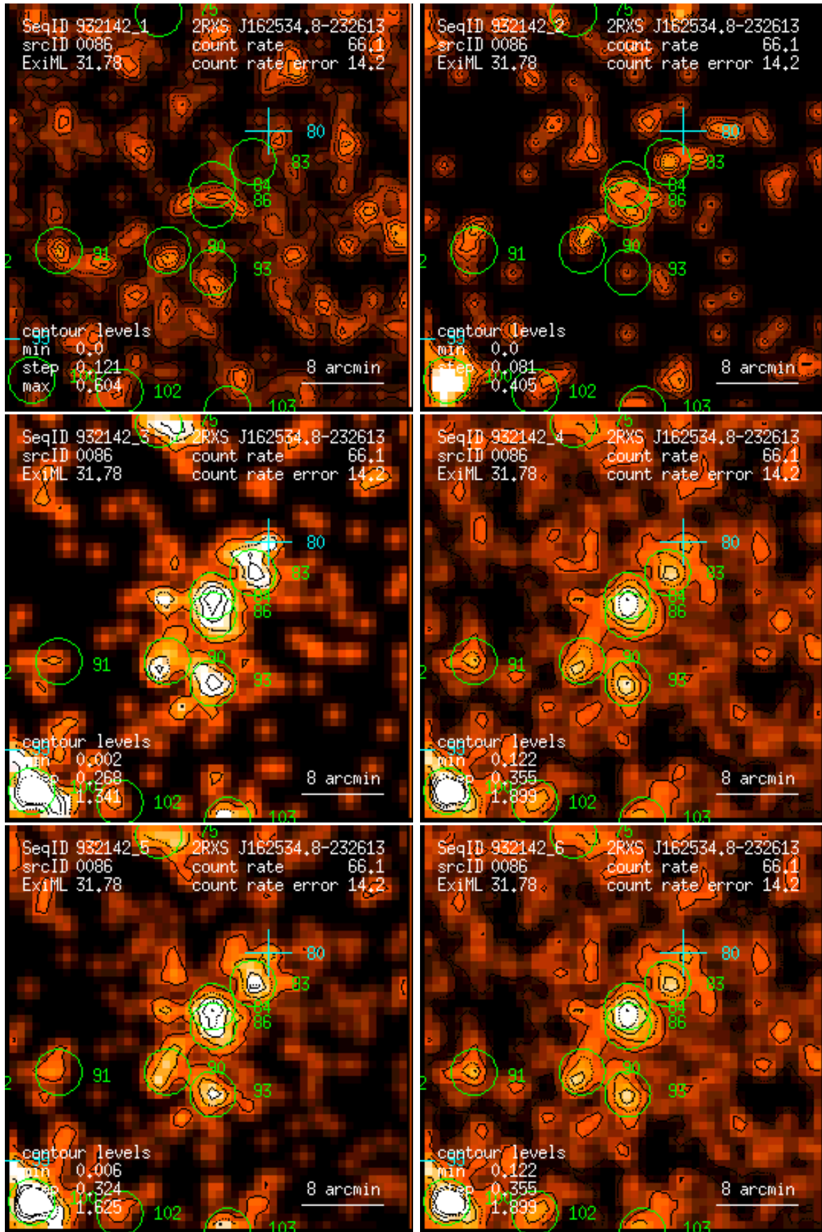
Figure 86: RASS 932142: detection 0086: band rate images, Gaussian filter: (1) PSPC channels 11 – 41, (2) 52 – 90, (3) 91 – 201, (4) 11 – 235, (5) 52 – 201, (6) 11 – 201. Broad band rates in counts/ks. Band rate contour levels in counts/ks/arcmin 2 .
