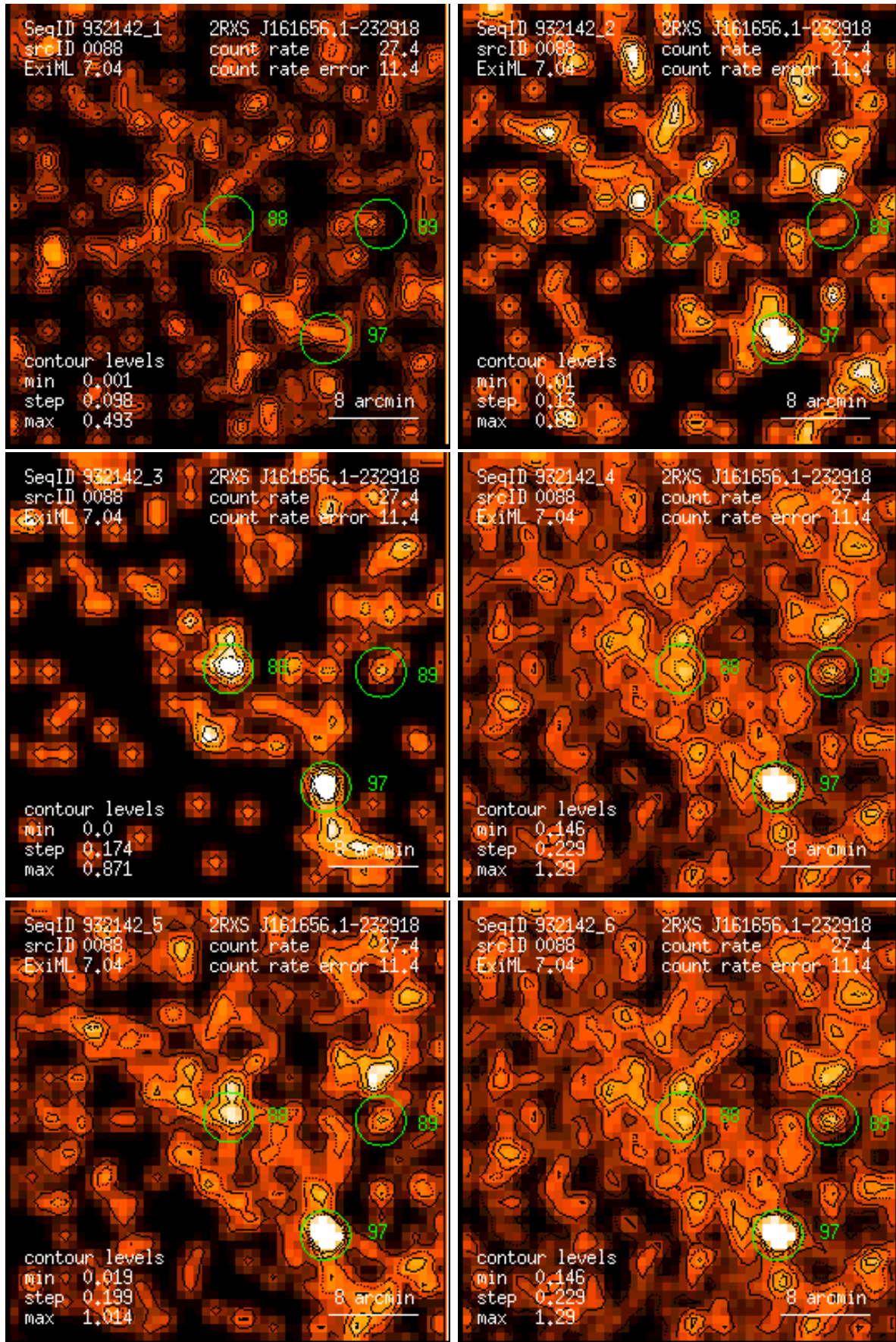
Figure 88: RASS 932142: detection 0088: band rate images, Gaussian filter: (1) PSPC channels 11 – 41, (2) 52 – 90, (3) 91 – 201, (4) 11 – 235, (5) 52 – 201, (6) 11 – 201. Broad band rates in counts/ks. Band rate contour levels in counts/ks/arcmin 2 .
