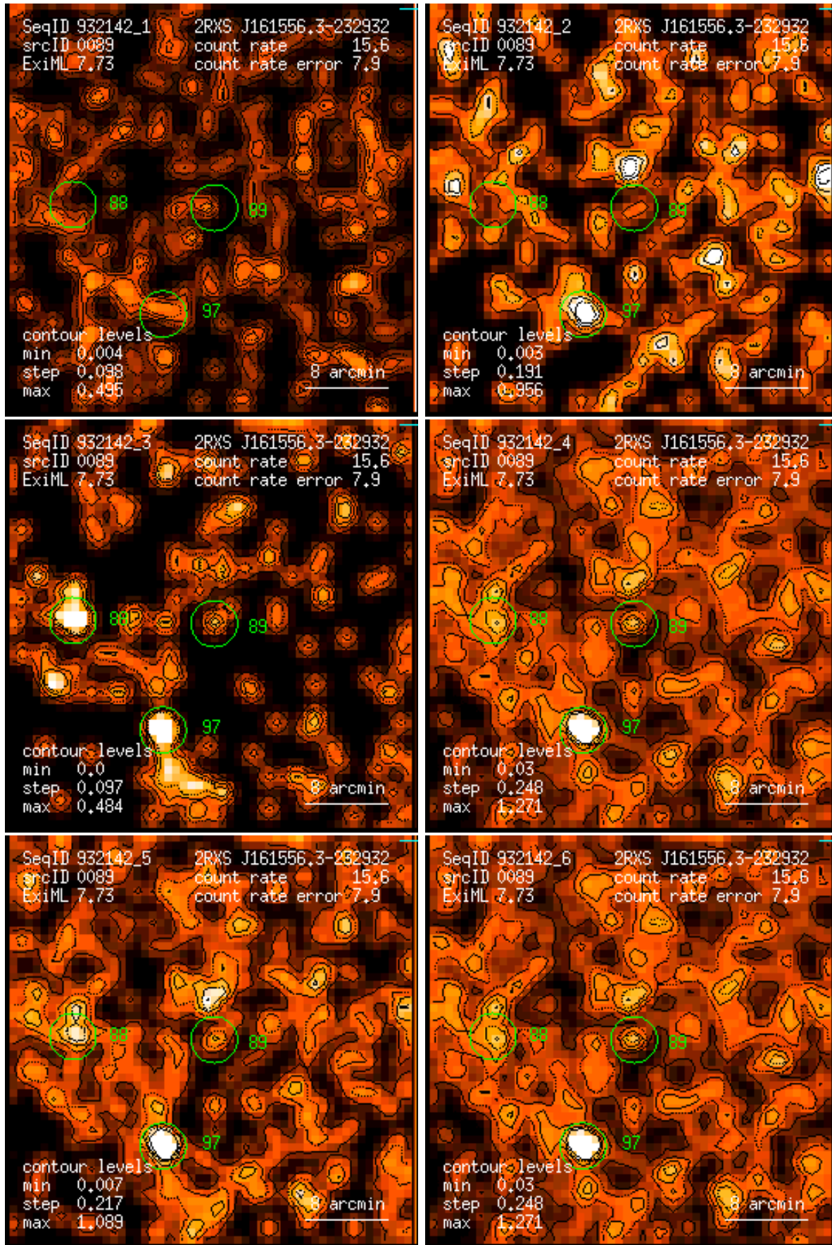
Figure 89: RASS 932142: detection 0089: band rate images, Gaussian filter: (1) PSPC channels 11 – 41, (2) 52 – 90, (3) 91 – 201, (4) 11 – 235, (5) 52 – 201, (6) 11 – 201. Broad band rates in counts/ks. Band rate contour levels in counts/ks/arcmin 2 .
