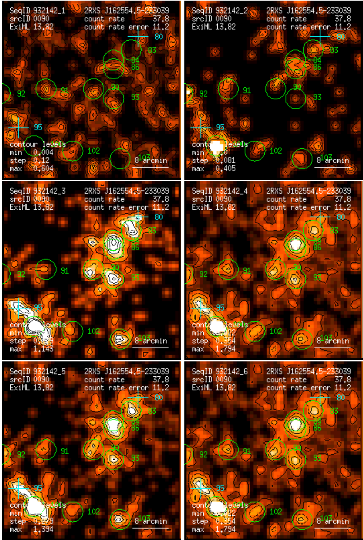
Figure 90: RASS 932142: detection 0090: band rate images, Gaussian filter: (1) PSPC channels 11 – 41, (2) 52 – 90, (3) 91 – 201, (4) 11 – 235, (5) 52 – 201, (6) 11 – 201. Broad band rates in counts/ks. Band rate contour levels in counts/ks/arcmin 2 .
