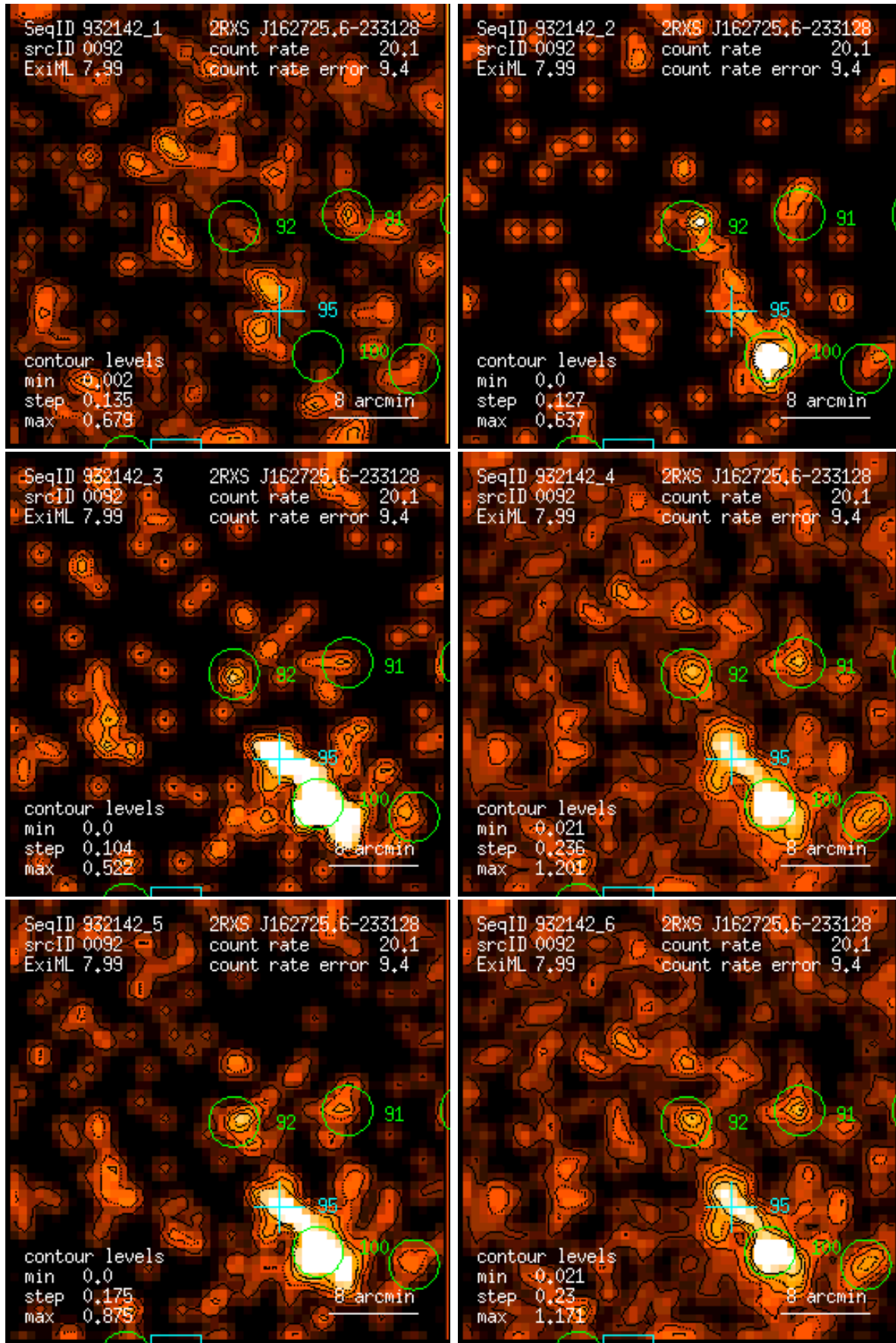
Figure 92: RASS 932142: detection 0092: band rate images, Gaussian filter: (1) PSPC channels 11 – 41, (2) 52 – 90, (3) 91 – 201, (4) 11 – 235, (5) 52 – 201, (6) 11 – 201. Broad band rates in counts/ks. Band rate contour levels in counts/ks/arcmin 2 .
