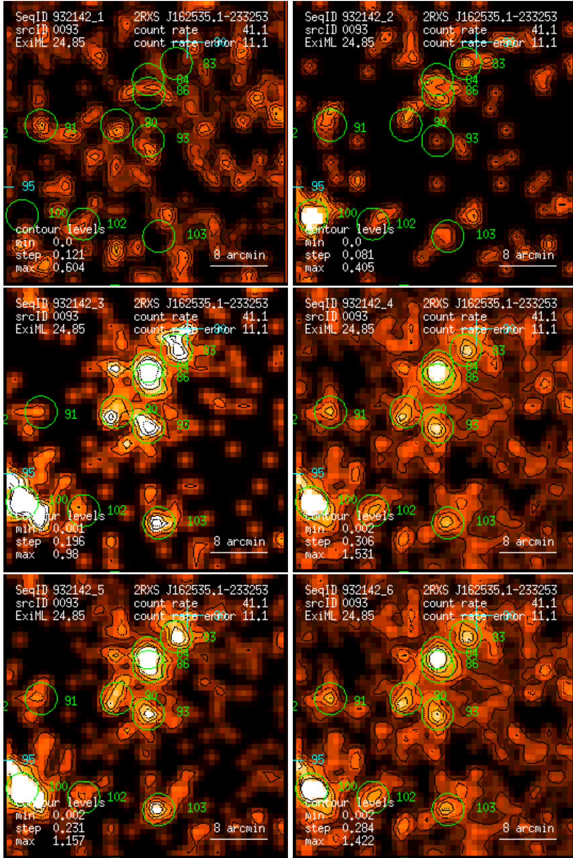
Figure 93: RASS 932142: detection 0093: band rate images, Gaussian filter: (1) PSPC channels 11 – 41, (2) 52 – 90, (3) 91 – 201, (4) 11 – 235, (5) 52 – 201, (6) 11 – 201. Broad band rates in counts/ks. Band rate contour levels in counts/ks/arcmin 2 .
