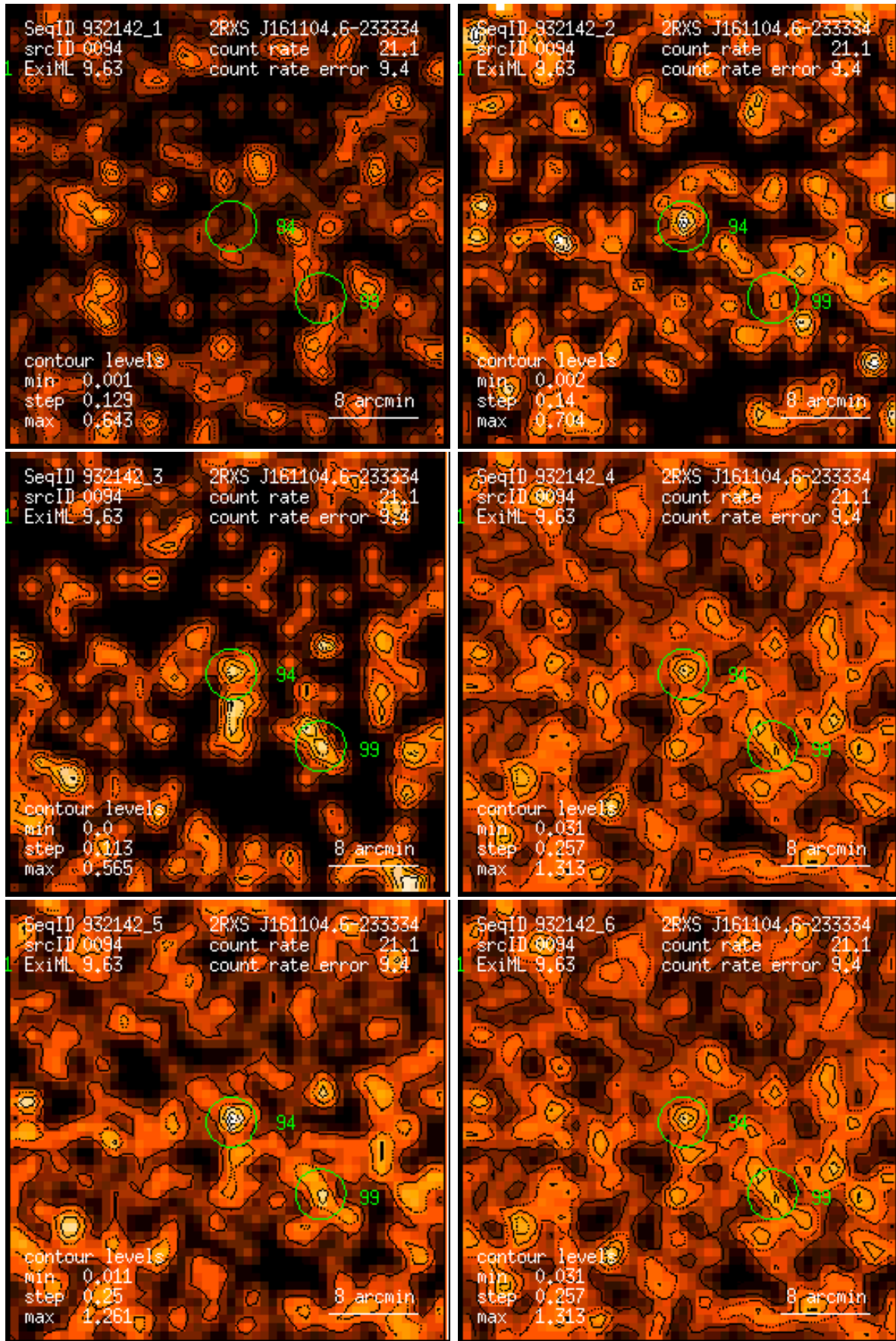
Figure 94: RASS 932142: detection 0094: band rate images, Gaussian filter: (1) PSPC channels 11 – 41, (2) 52 – 90, (3) 91 – 201, (4) 11 – 235, (5) 52 – 201, (6) 11 – 201. Broad band rates in counts/ks. Band rate contour levels in counts/ks/arcmin 2 .
