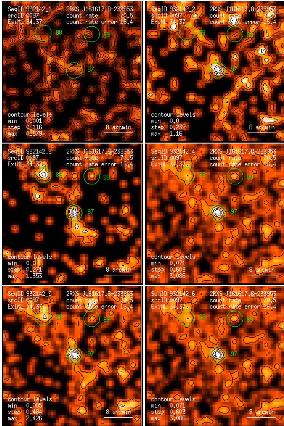
Figure 97: RASS 932142: detection 0097: band rate images, Gaussian filter: (1) PSPC channels 11 – 41, (2) 52 – 90, (3) 91 – 201, (4) 11 – 235, (5) 52 – 201, (6) 11 – 201. Broad band rates in counts/ks. Band rate contour levels in counts/ks/arcmin 2 .
