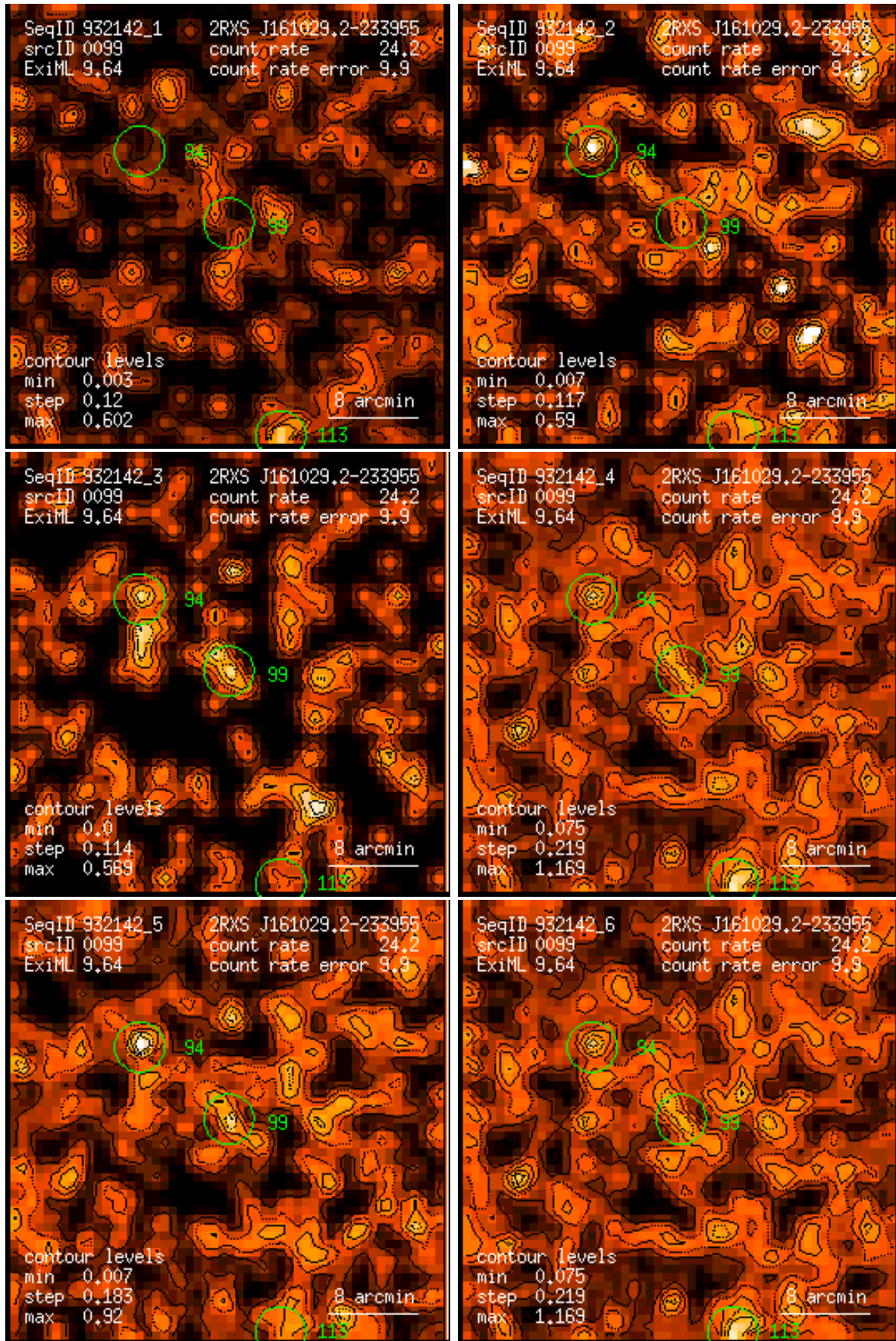
Figure 99: RASS 932142: detection 0099: band rate images, Gaussian filter: (1) PSPC channels 11 – 41, (2) 52 – 90, (3) 91 – 201, (4) 11 – 235, (5) 52 – 201, (6) 11 – 201. Broad band rates in counts/ks. Band rate contour levels in counts/ks/arcmin 2 .
