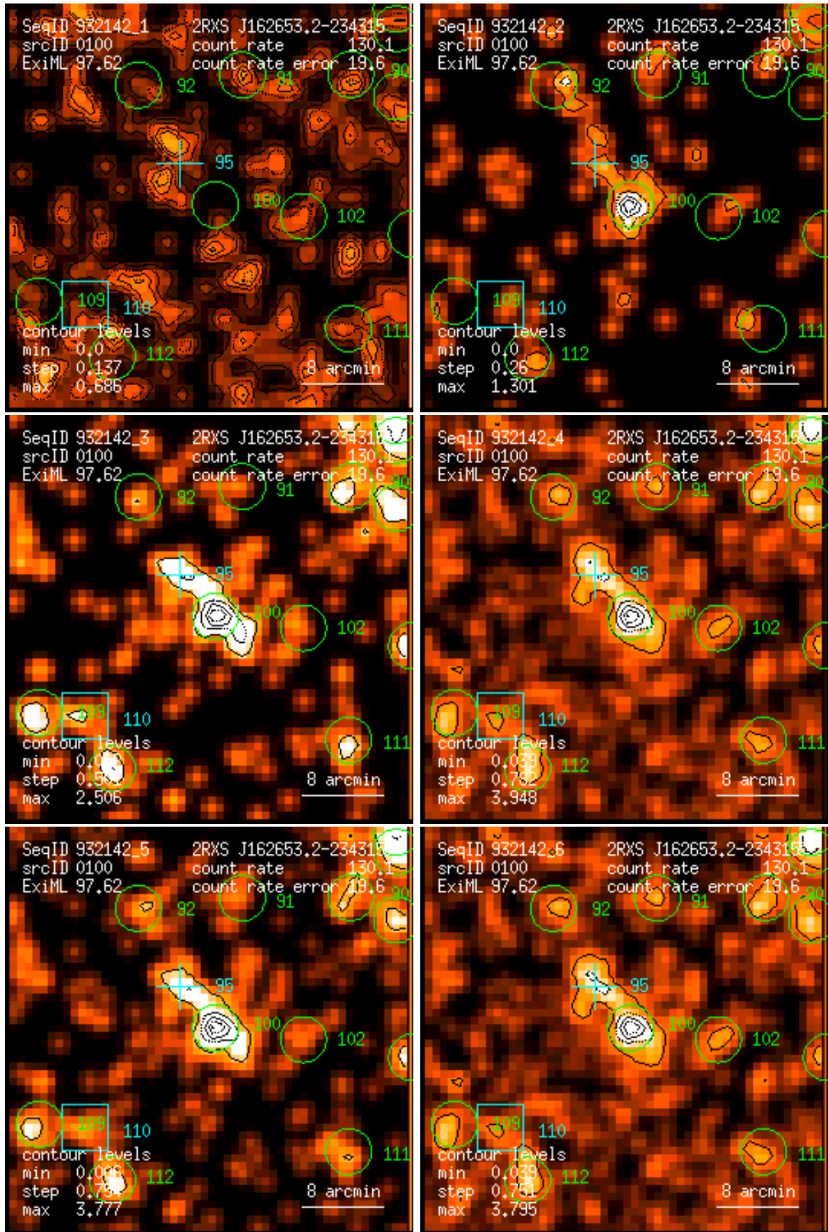
Figure 100: RASS 932142: detection 0100: band rate images, Gaussian filter: (1) PSPC channels 11 – 41, (2) 52 – 90, (3) 91 – 201, (4) 11 – 235, (5) 52 – 201, (6) 11 – 201. Broad band rates in counts/ks. Band rate contour levels in counts/ks/arcmin 2 .
