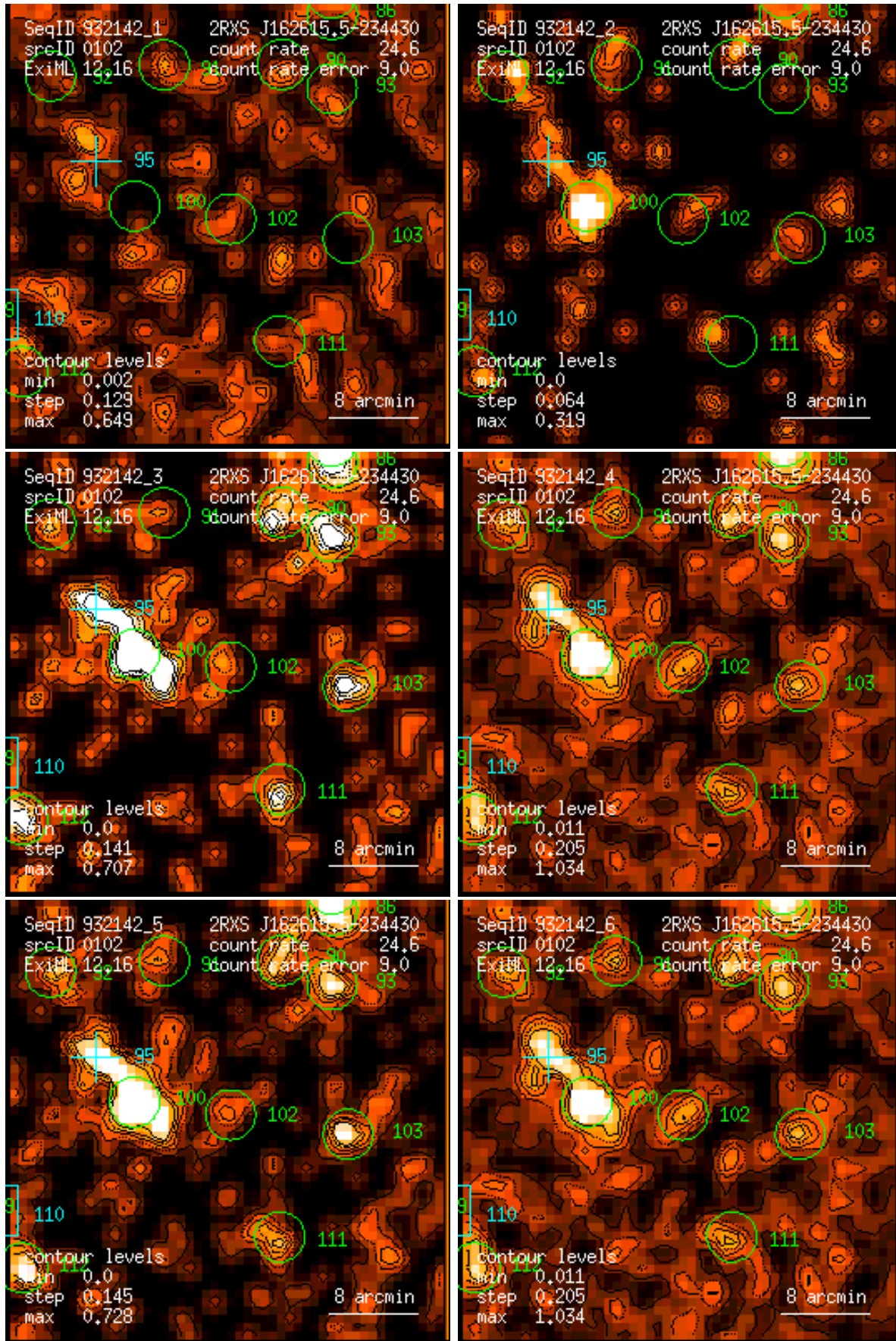
Figure 102: RASS 932142: detection 0102: band rate images, Gaussian filter: (1) PSPC channels 11 – 41, (2) 52 – 90, (3) 91 – 201, (4) 11 – 235, (5) 52 – 201, (6) 11 – 201. Broad band rates in counts/ks. Band rate contour levels in counts/ks/arcmin 2 .
