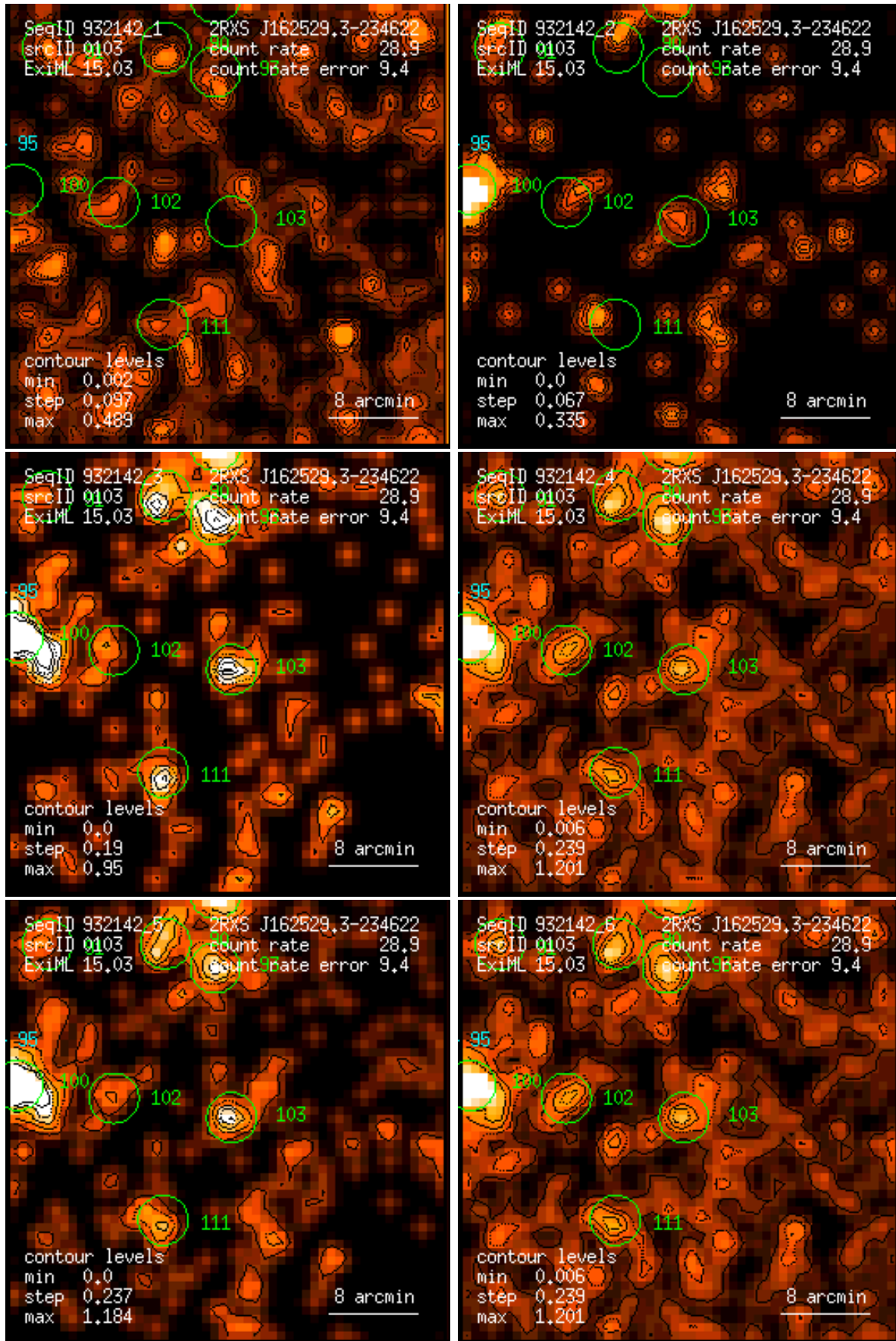
Figure 103: RASS 932142: detection 0103: band rate images, Gaussian filter: (1) PSPC channels 11 – 41, (2) 52 – 90, (3) 91 – 201, (4) 11 – 235, (5) 52 – 201, (6) 11 – 201. Broad band rates in counts/ks. Band rate contour levels in counts/ks/arcmin 2 .
